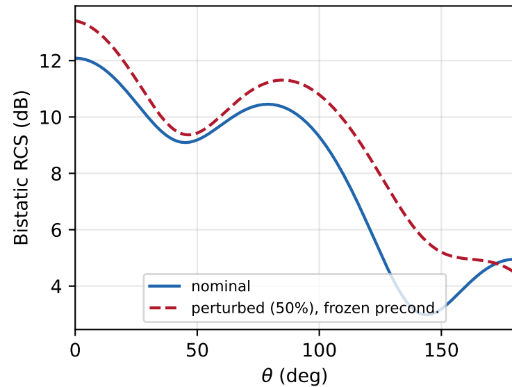
Sphere
