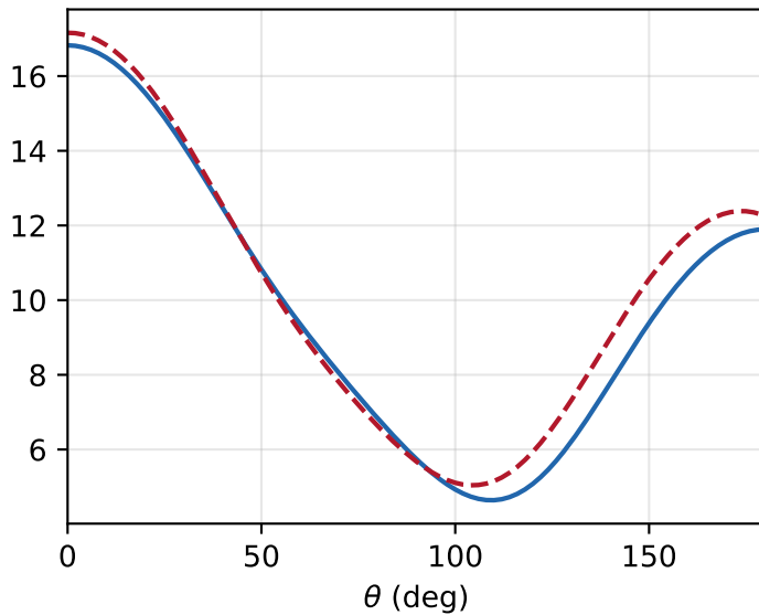
Ellipsoid
