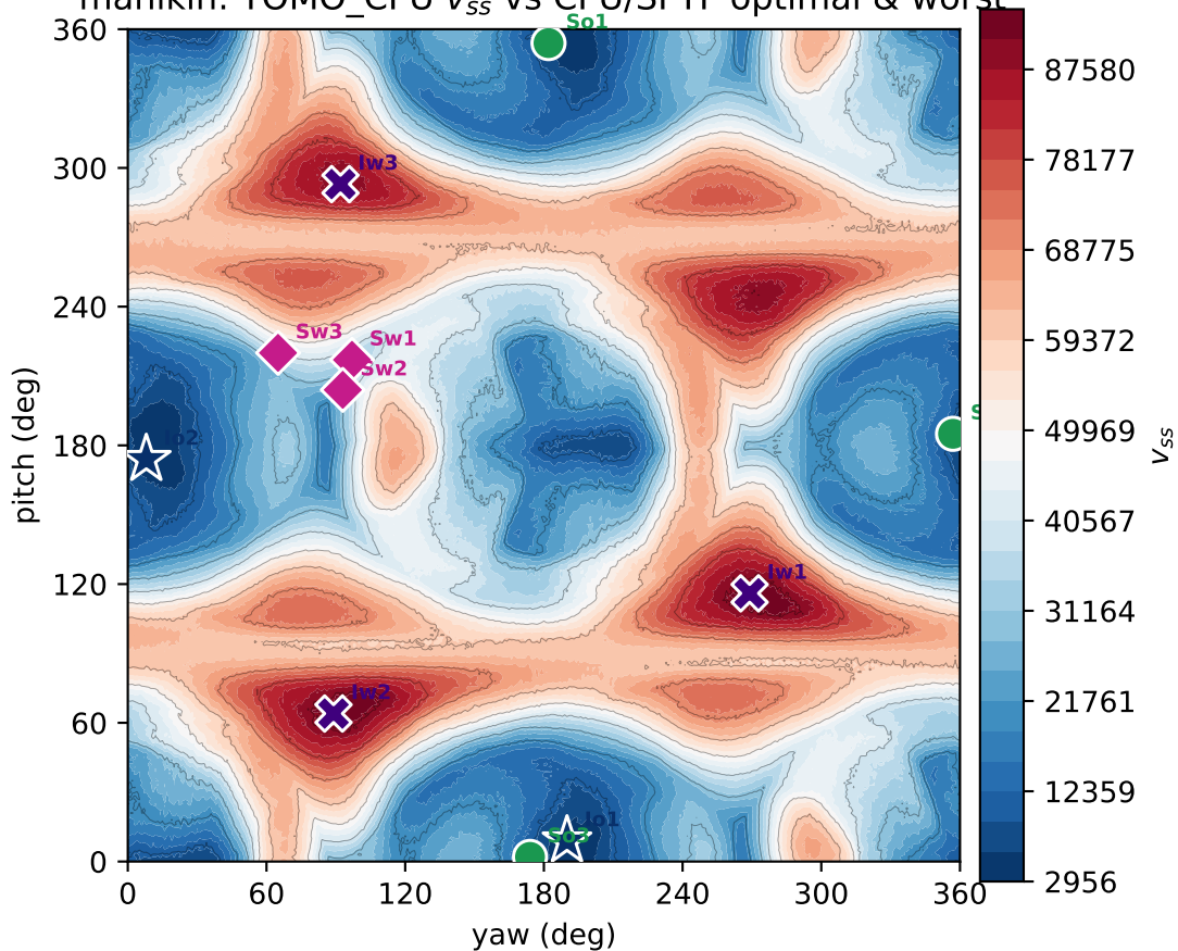
manikin: TOMO_CPU v_{ss} vs CPU/SFTF optimal & worst
