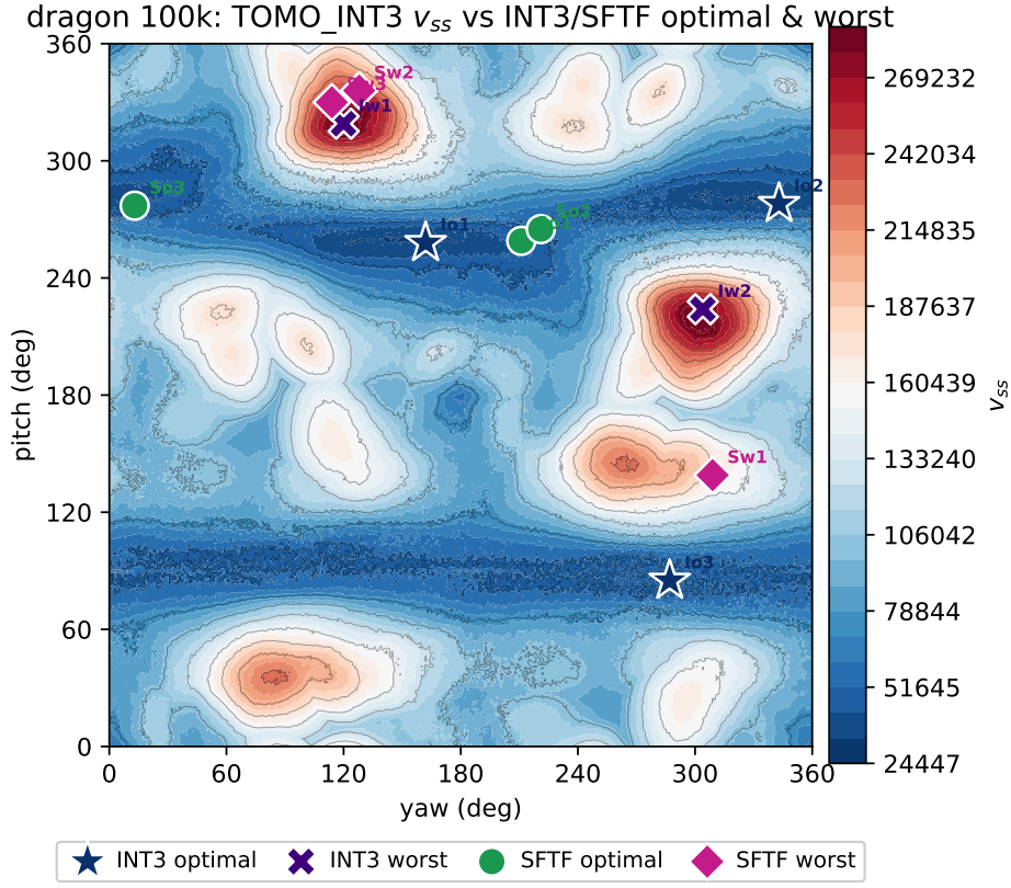
Fig. 11 Comparison of INT3/SFTF optimal/worst orientations on the TOMO_INT3 v_{ss} landscape of dragon 100k (blue is good). The markers are 3 each of INT3/SFTF optimal/worst, with kinds following the legend below the figure. The global optimum is v_{ss} = 24447 (yaw= 162°, pitch= 258°), and the absolute v_{ss} scale is large due to the abundant surface detail, but the global optimum forms a relatively distinct basin.
