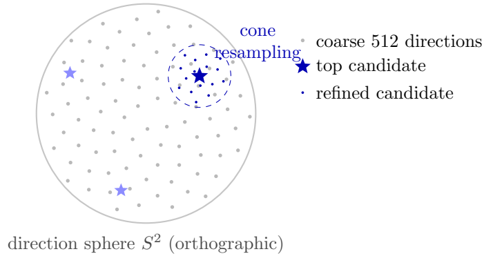
Fig. 3 Two-stage direction search. After evaluating coarse candidates (gray, 512) that sparsely cover the sphere via the Fibonacci sphere, the regions around the top candidates (stars) are densely resampled with 2^\circ – 8^\circ cones (blue dots) to reflect sensitivity near the optimal direction. Local precision is obtained without densely evaluating the entire sphere.
