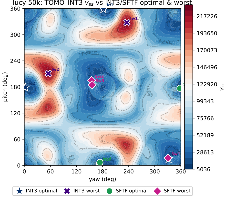
Fig. 13 Comparison of INT3/SFTF optimal/worst orientations on the TOMO_INT3 v_{ss} landscape of lucy 50k (blue is good). The markers are 3 each of INT3/SFTF optimal/worst, with kinds following the legend below the figure. The global optimum is v_{ss} = 5036 (yaw= 182°, pitch= 359°), and being located near the pitch boundary (359°), it requires basin search that considers the yaw–pitch periodicity.
