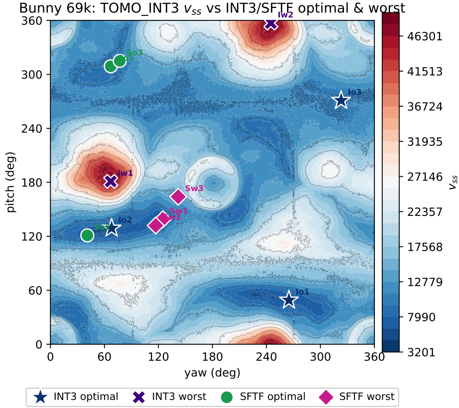
Fig. 9 Comparison of INT3/SFTF optimal/worst orientations on the TOMO_INT3 v_{ss} landscape of Bunny 69k (blue is good). The markers are 3 each of INT3/SFTF optimal/worst, with kinds following the legend below the figure. The global optimum is v_{ss} = 3201 (yaw= 265^\circ , pitch= 49^\circ ; Table 1 in the main text), and lies not at a single point but within a broad low-cost basin.
