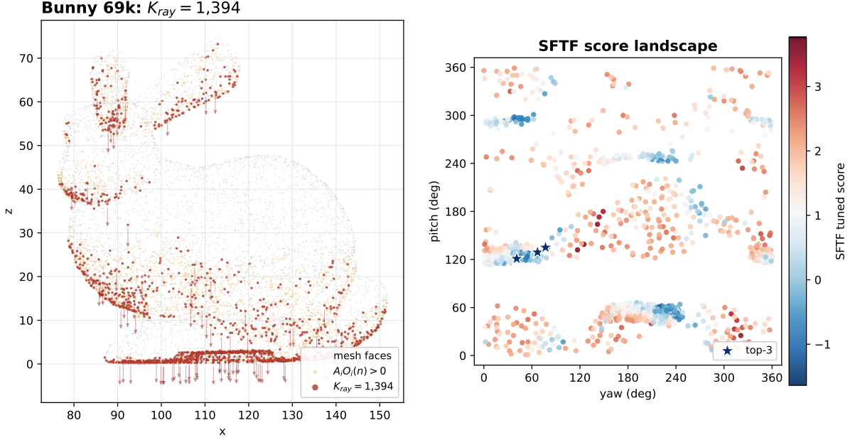
Fig. 7 Bunny 69k source-face sampling and SFTF score landscape with the adaptive rule, K_{ray} = \text{clip}(0.02N_f, 500, 3000) = 1,394 .
