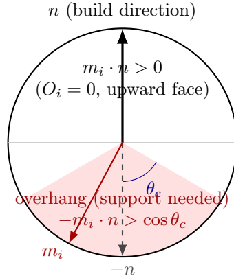
Fig. 2 Geometric meaning of the overhang coefficient O_i(n) = \max(0, -m_i \cdot n) . The possible face-normal directions are shown on a unit circle with respect to the build direction n . The upper semicircle ( m_i \cdot n > 0 ) consists of upward faces with O_i = 0 , and the lower shaded region is the cone of half-angle \theta_c around -n , where faces with -m_i \cdot n > \cos \theta_c are overhangs that actually require support. O_i grows the more the normal aligns with -n (the further down it goes).
