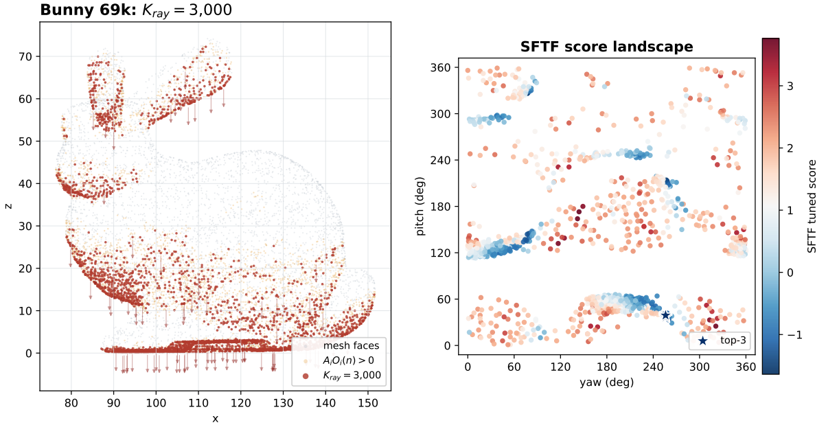
Fig. 8 Bunny 69k source-face sampling and SFTF score landscape with fixed K_{ray} = 3000 , corresponding to the upper cap used for large meshes.
