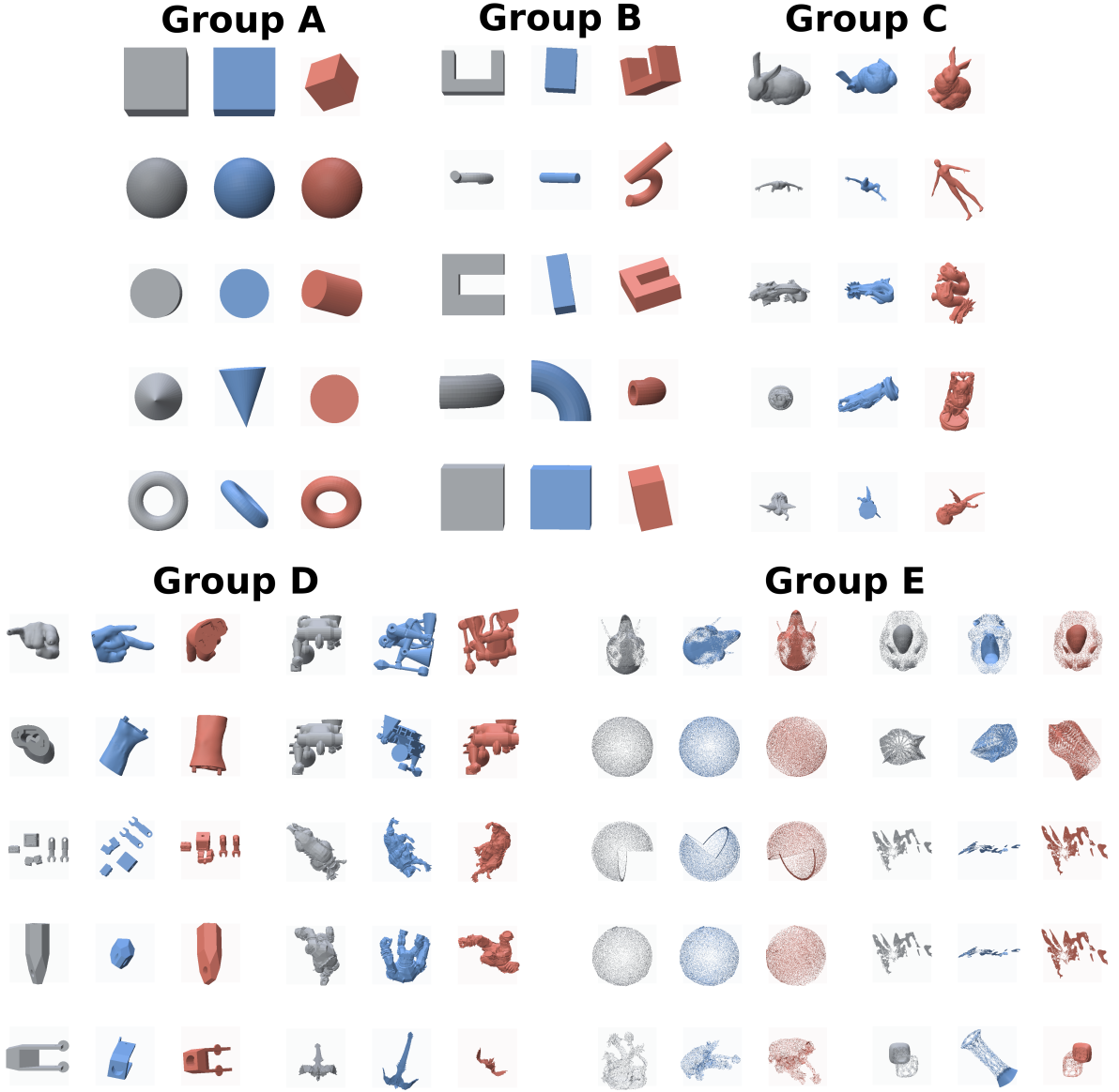
Fig. 5 Best/worst build-orientation Polyscope overlay arranged by group for the five groups (A–E) ( \theta_c = 60^\circ ). A label is placed atop each group, with groups A–C in the top row and groups D/E (a vertical 5-row 2-column layout each) in the bottom row, grouped about the page center. Each mesh shows the original (gray), optimal orientation (blue), and worst orientation (red) side by side, displayed in the actual print pose by rotating the stored build direction to world +Z . Since SFTF candidates are invariant to \theta_c , the overlays of the five critical angles are identical.
