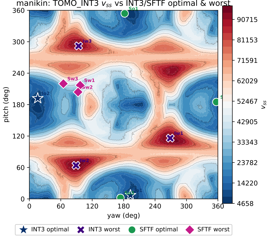
Fig. 10 Comparison of INT3/SFTF optimal/worst orientations on the TOMO_INT3 v_{ss} landscape of manikin (blue is good). The markers are 3 each of INT3/SFTF optimal/worst, with kinds following the legend below the figure. The global optimum is v_{ss} = 4658 (yaw= 193^\circ , pitch= 7^\circ ), and befitting a vertically elongated shape, the low-cost region is distributed in a narrow pitch band across the full yaw range.
