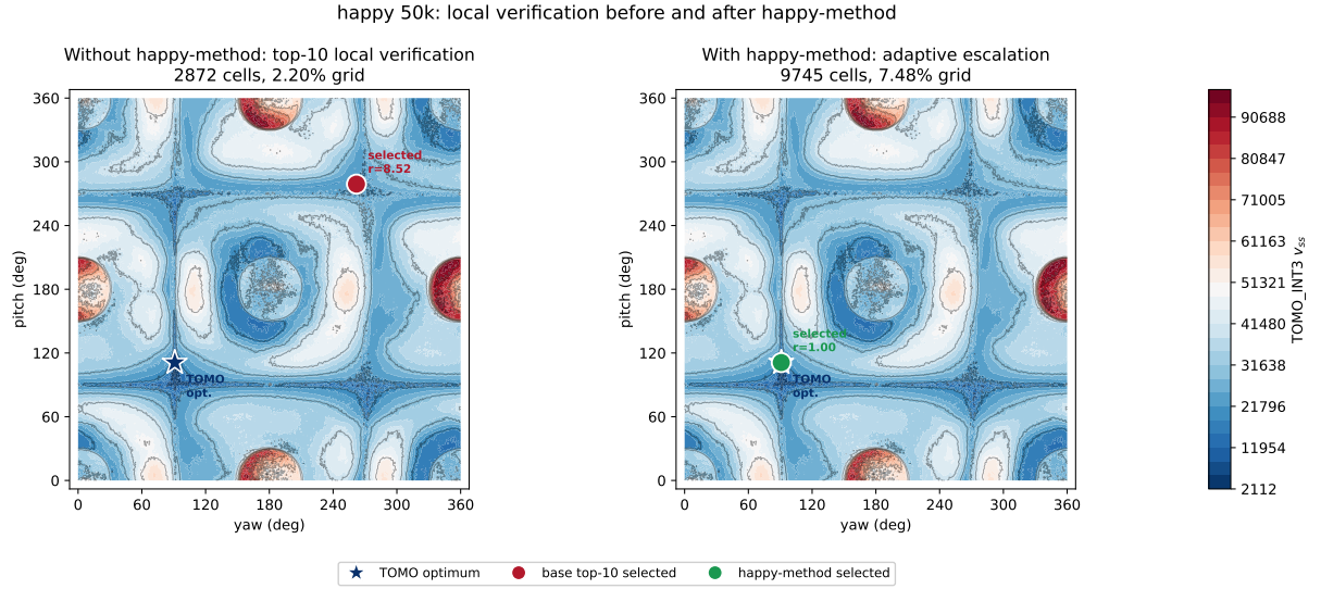
Fig. 12 happy 50k before and after happy-method escalation on the same TOMO_INT3 v_{ss} landscape. Without escalation, the base top-10 local verification selects a high-cost basin ( v_{ss} = 17,991 , ratio 8.52, 2.20% grid budget). With the happy-method trigger, the search is expanded to the adaptive final set and recovers the TOMO optimum ( v_{ss} = 2,112 , ratio 1.00, 7.48% grid budget). This visualizes why happy is treated as a local-verification hard case rather than as a score-weight tuning failure.
