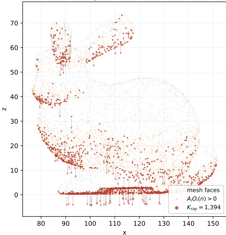
Bunny 69k: K_{ray} = 1,394
