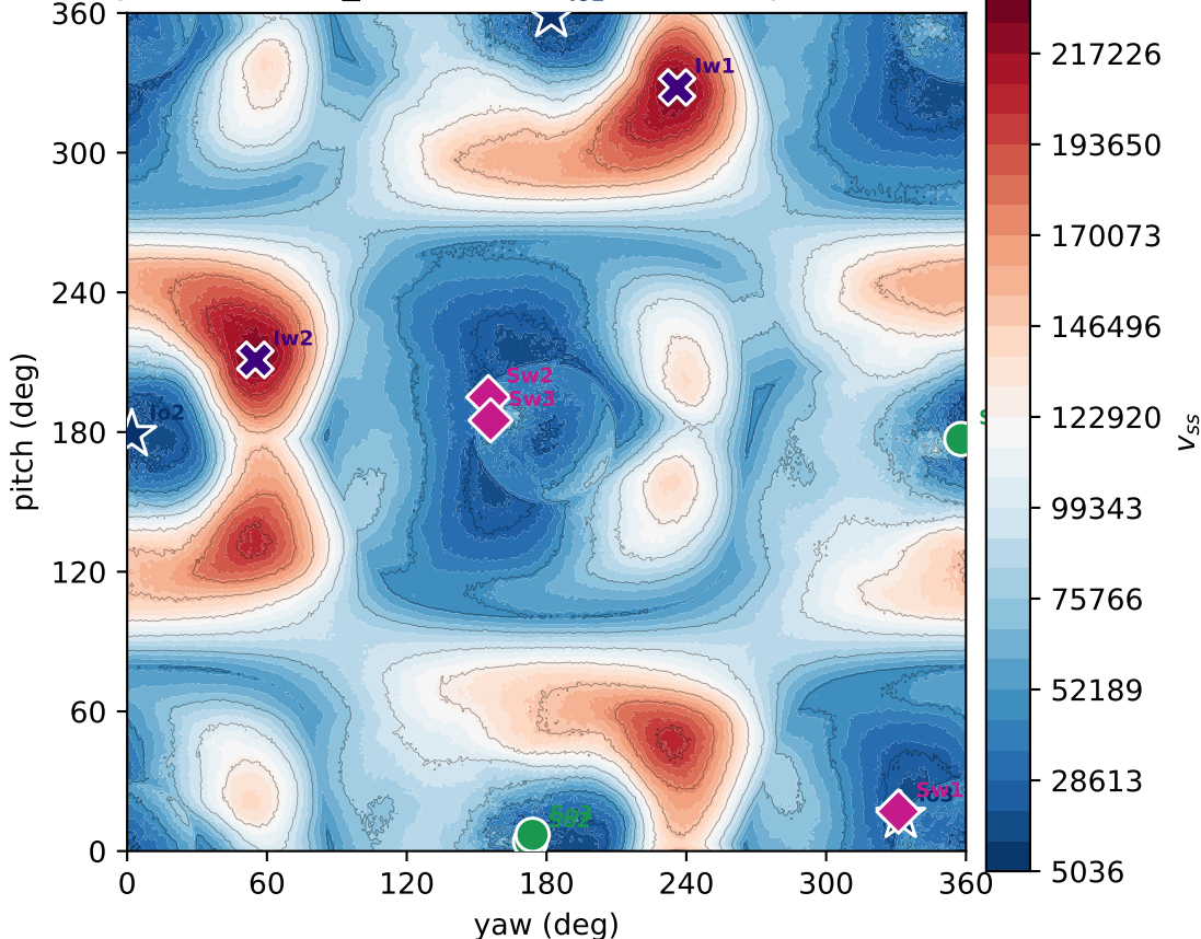
lucy 50k: TOMO_INT3 v_{ss} vs INT3/SFTF optimal & worst
