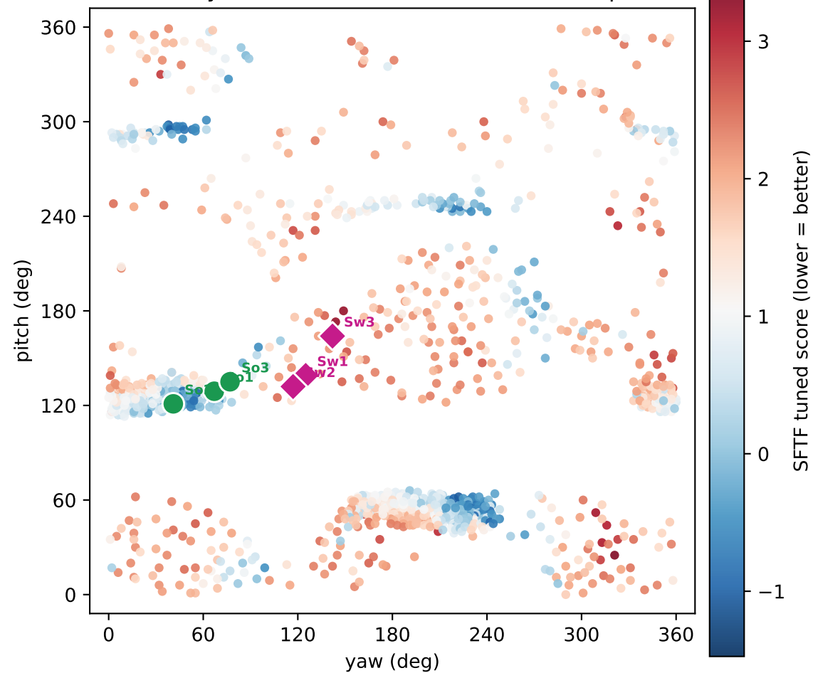
Bunny 69k: SFTF candidate cost landscape
