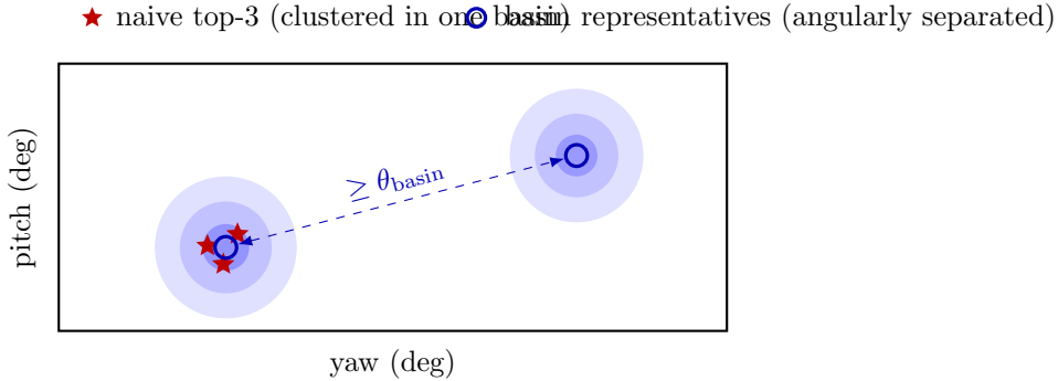
Figure 5: Top- k points vs. Top- k basins. When there are several mutually separated low-cost basins (blue regions) on the yaw-pitch cost landscape, simply picking the top points with small v_{ss} (red stars) repeatedly selects only neighboring points within one basin. With angular non-maximum suppression (NMS), keeping only candidates that are at least \theta_{\text{basin}} away from the already-chosen representatives (blue circles), different near-optimal orientation groups are presented as representatives.
