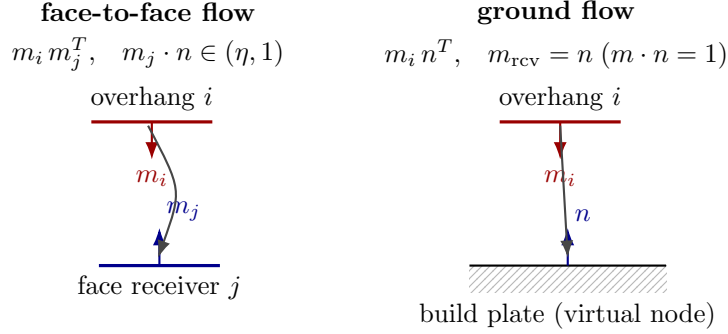
Figure 2: The two flow terms of the unified tensor. (Left) When overhang i is supported by an actual face j , the receiver normal is m_j \cdot n \in (\eta, 1) and the tensor term is m_i m_j^T . (Right) When there is no face to support it, it is supported by the build plate, “a limiting receiver whose normal is exactly n ” ( m \cdot n = 1 ), and the term becomes m_i n^T . The build-plate cost B(n) is exactly equal to the Rayleigh contribution of this ground term (Eq. (18)).
