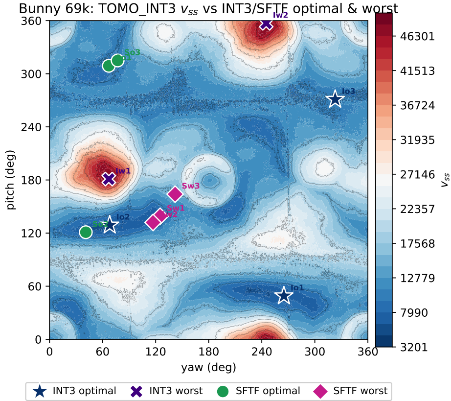
Figure 10: Comparison of INT3/SFTF optimal/worst orientations on the TOMO_INT3 v_{ss} landscape of Bunny 69k (blue is good). The markers are 3 each of INT3/SFTF optimal/worst, with kinds following the legend below the figure. The global optimum is v_{ss} = 3201 (yaw= 265^\circ , pitch= 49^\circ ; Table 1 in the main text), and lies not at a single point but within a broad low-cost basin.
