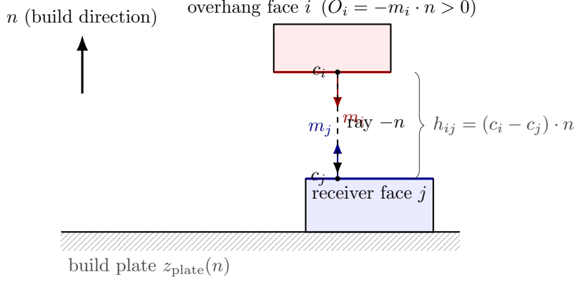
Figure 1: Geometry of the support flow. From overhang face i (downward normal m_i , O_i = \max(0, -m_i \cdot n) > 0 ), a ray is cast in -n , opposite the build direction, to find the valid receiver face j below. A support flow is recognized only when the height difference h_{ij} = (c_i - c_j) \cdot n > 0 , and this face-to-face pair forms one term of the tensor F(n) = \sum w_{ij} A_i A_j m_i m_j^T .
