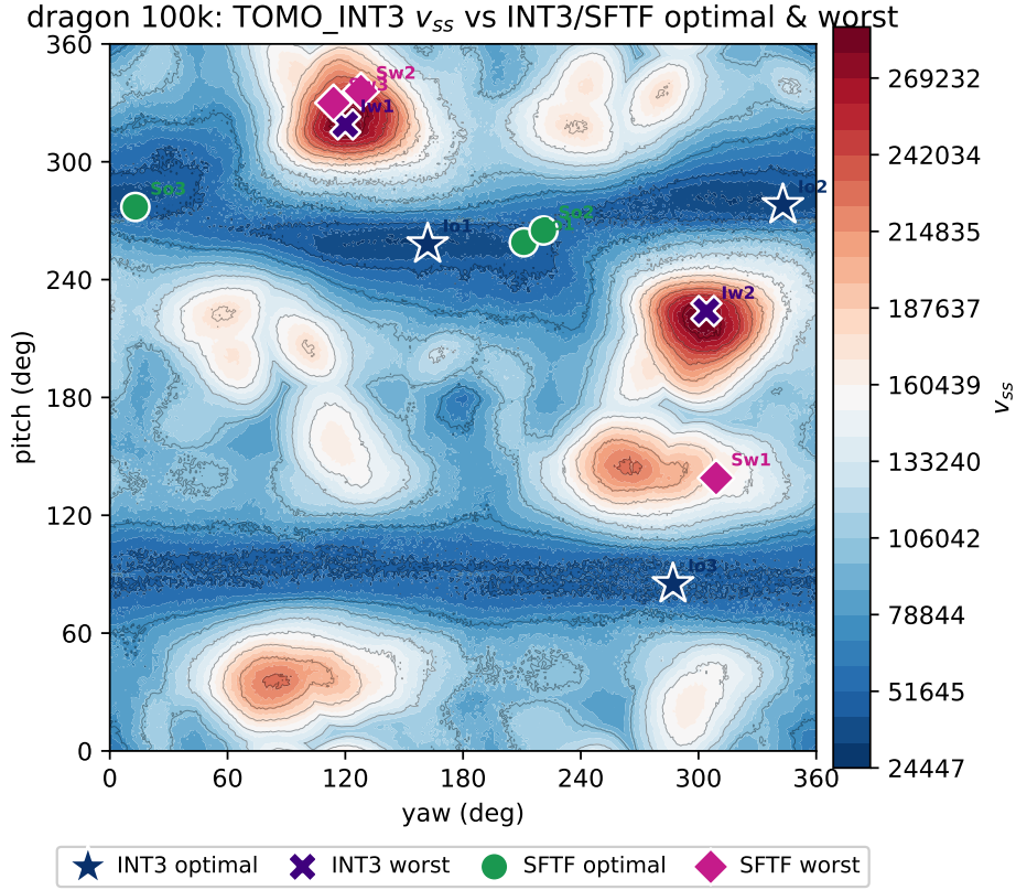
Figure 12: Comparison of INT3/SFTF optimal/worst orientations on the TOMO_INT3 v_{ss} landscape of dragon 100k (blue is good). The markers are 3 each of INT3/SFTF optimal/worst, with kinds following the legend below the figure. The global optimum is v_{ss} = 24447 (yaw= 162°, pitch= 258°), and the absolute v_{ss} scale is large due to the abundant surface detail, but the global optimum forms a relatively distinct basin.
