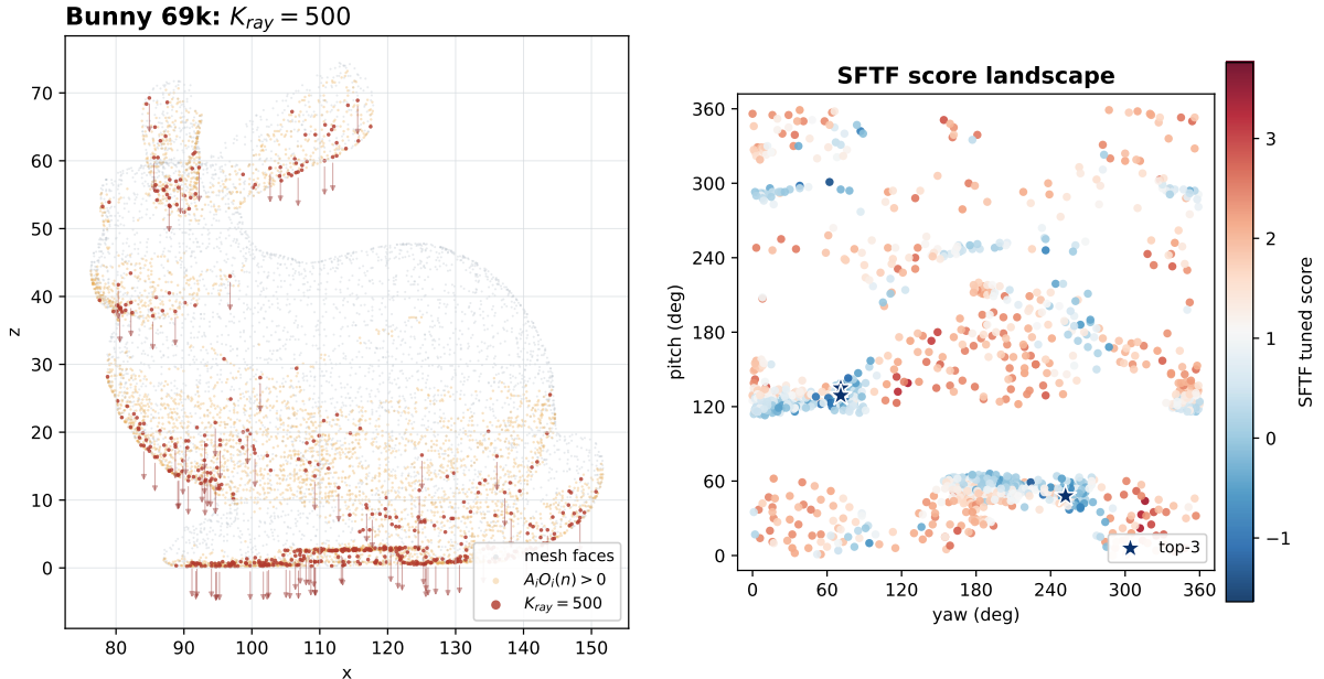
Figure 7: Bunny 69k source-face sampling and SFTF score landscape with fixed K_{ray} = 500 . The right panel is recomputed with the same ray budget and uses the common color scale of Figures 8–9.
