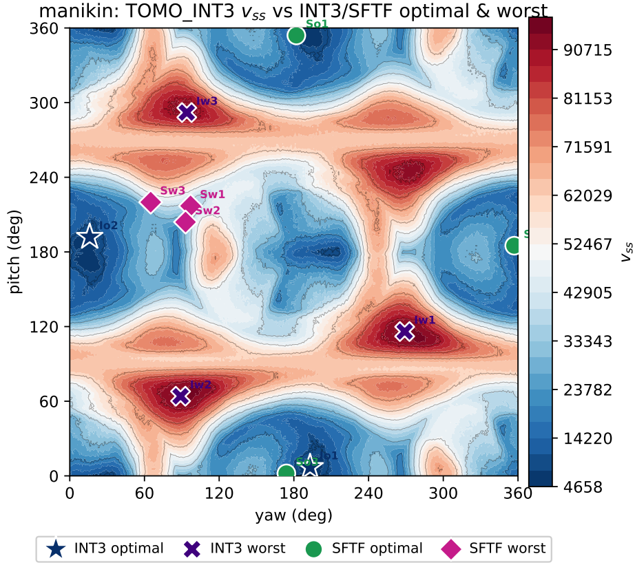
Figure 11: Comparison of INT3/SFTF optimal/worst orientations on the TOMO_INT3 v_{ss} landscape of manikin (blue is good). The markers are 3 each of INT3/SFTF optimal/worst, with kinds following the legend below the figure. The global optimum is v_{ss} = 4658 (yaw= 193^\circ , pitch= 7^\circ ), and befitting a vertically elongated shape, the low-cost region is distributed in a narrow pitch band across the full yaw range.
