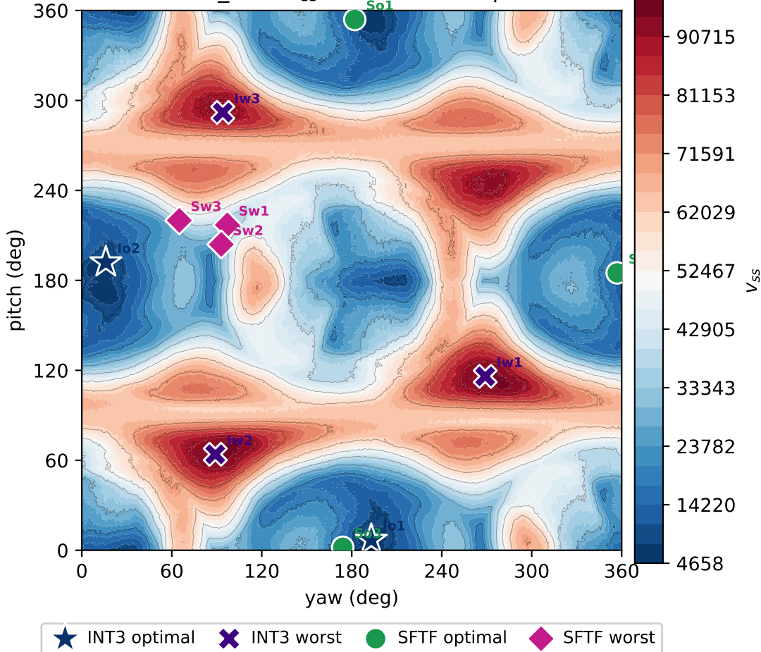
manikin: TOMO_INT3 v_{ss} vs INT3/SFTF optimal & worst
