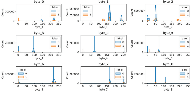
Fig. 3: Feature distribution by label
