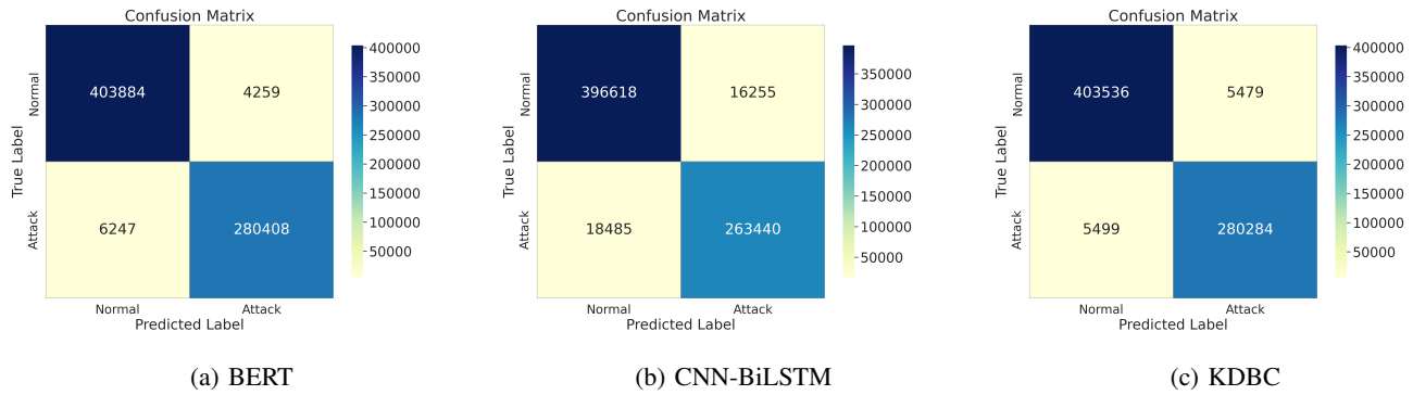
Fig. 12: The confusion matrix of three models on real vehicle test
