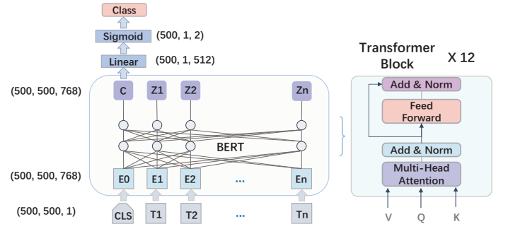
Fig. 5: The structure of BERT model
