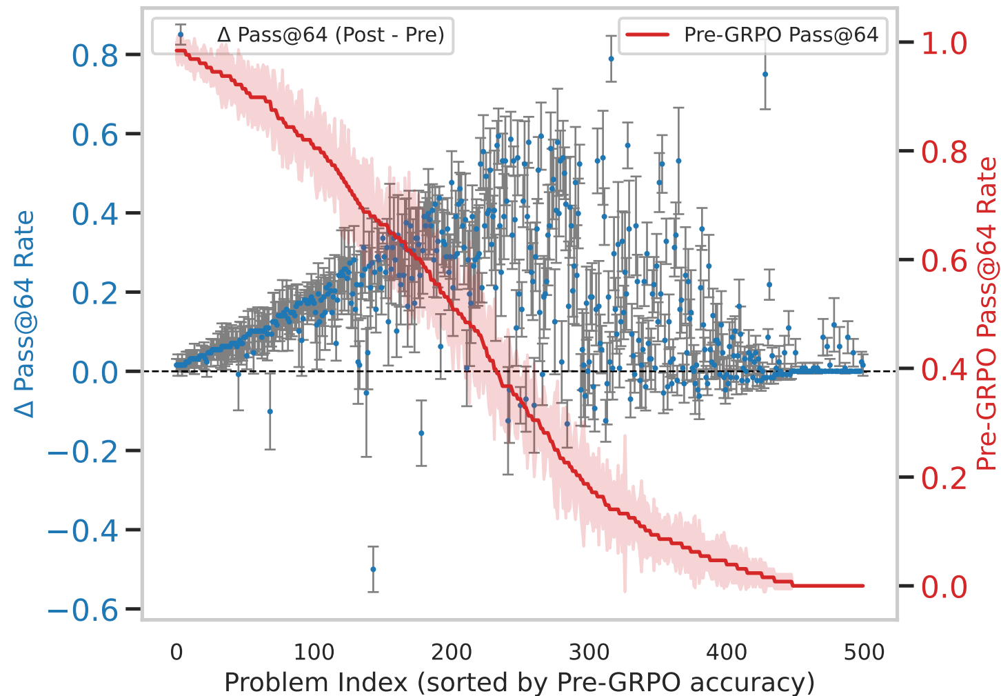
GRPO Gains vs Pre-GRPO Baseline
