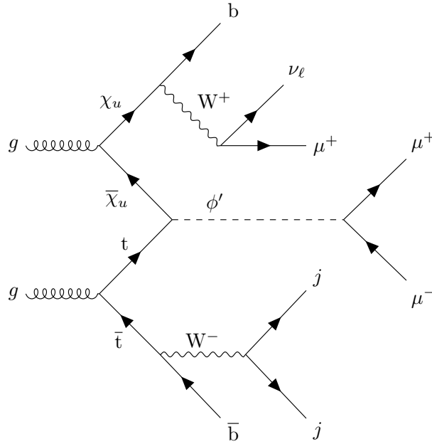
Figure 3.3: Representative Feynman diagram for the production of a \phi' boson in association with a \chi_u vector-like quark through the fusion of a top quark and \chi_u vector-like quark. Once again, the \phi' decays to a pair of muons, the top quark decays fully hadronically, and the \chi_u decays semi-leptonically to muons, neutrinos and b-jets.
