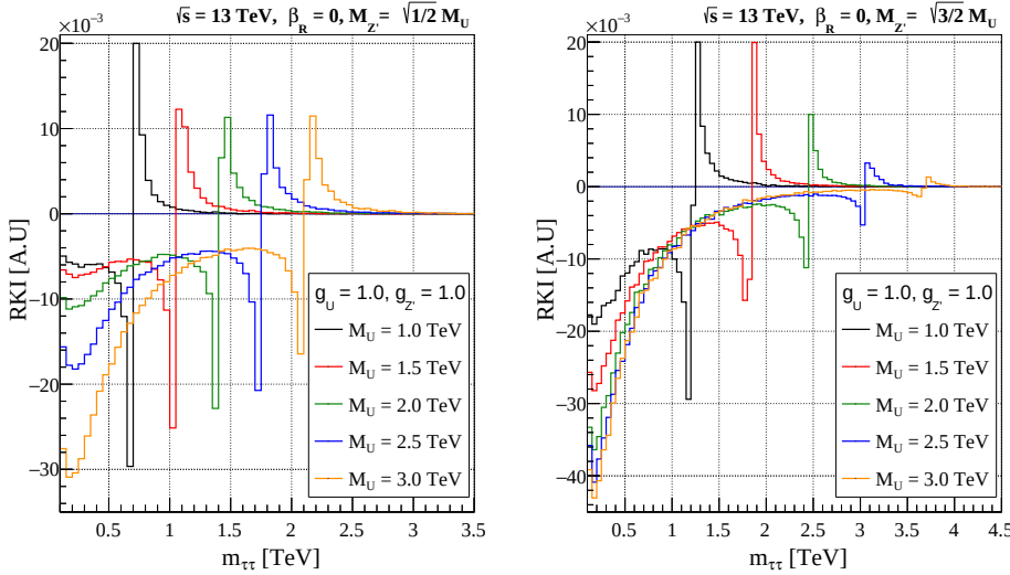
Figure 4.4: Relative kinematic interference (RKI) versus reconstructed di-tau invariant mass for various LQ masses, calculated at \sqrt{s} = 13 TeV with \beta_R = 0 , g_U = 1.0 , g_{Z'} = 1.0 . Left: M_{Z'} = \sqrt{1/2} M_U . Right: M_{Z'} = \sqrt{3/2} M_U .
