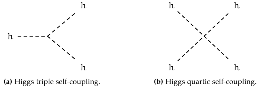
Figure 1.6: Feynman diagrams for Higgs self-interactions arising from the potential V(H^\dagger, H) = -\mu^2|H|^2 + \lambda|H|^4 in the Higgs Lagrangian.
