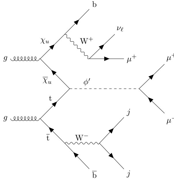
Figure 3.3: Feynman diagram Representing \phi' boson production accompanied by a \chi_u vector-like quark via top quark and \chi_u fusion. The diagram shows \phi' decay to muon pairs, hadronic top quark decay, and semi-leptonic \chi_u decay producing muons, neutrinos, and b-jets.
