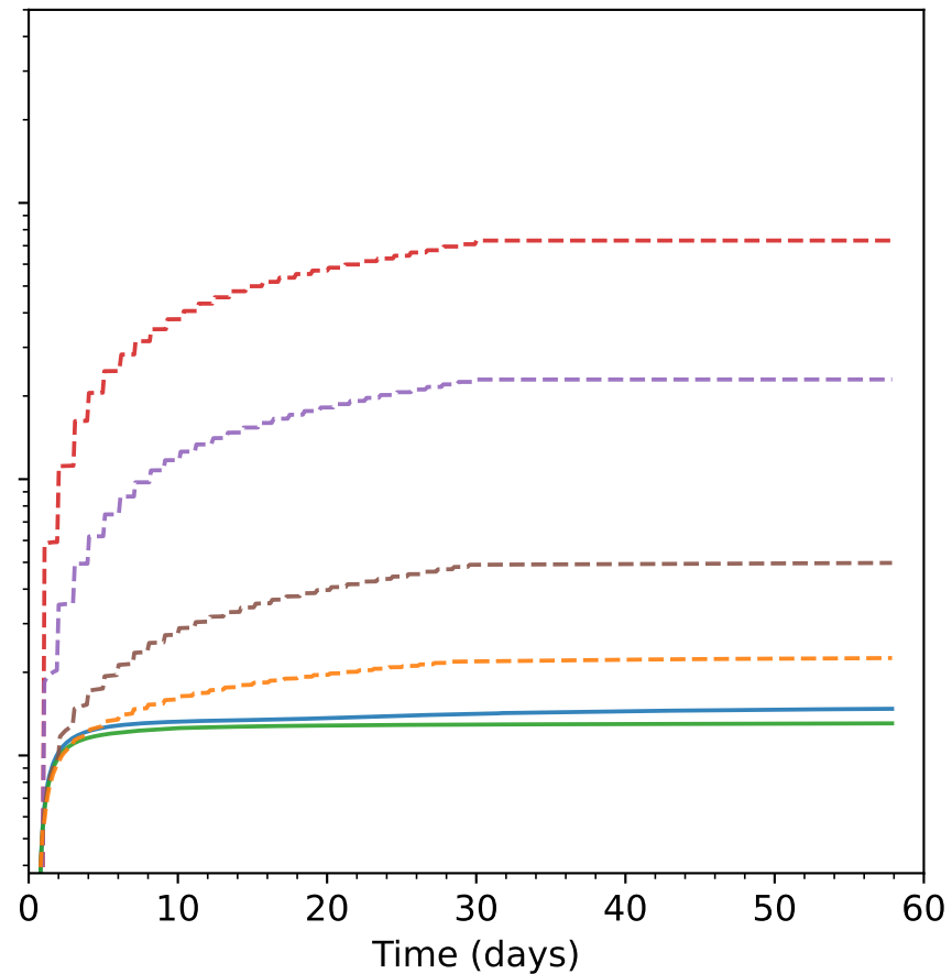
Photosphere shell ( m = 4.94 M_{\odot} )
