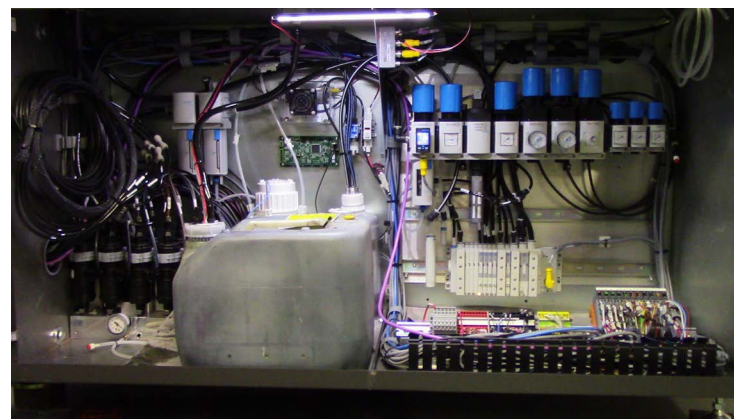
Figure 7-2 Waste compartment
