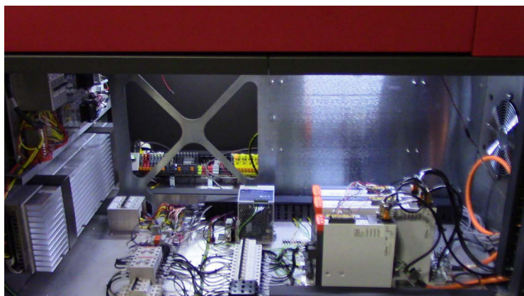
Figure 7-1 Motion compartment
