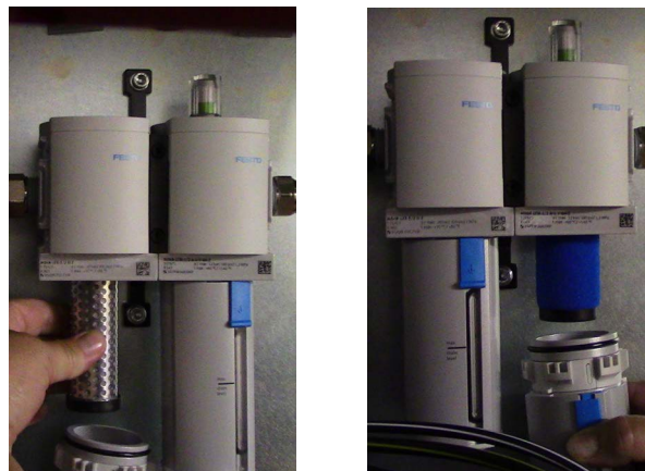
Figure 8-13 Carbon filter, LEFT, and Micro Filter, RIGHT
