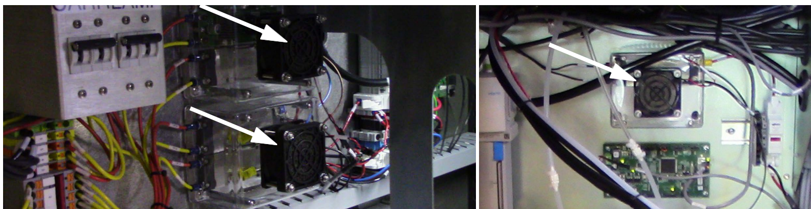
Figure 6-11 Additional Power Supply Fans, Electronics Compartment, Left, and Waste Compartment, Right
