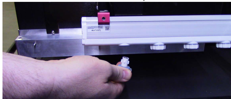
Figure 6-16 Removing Static Eliminator head
