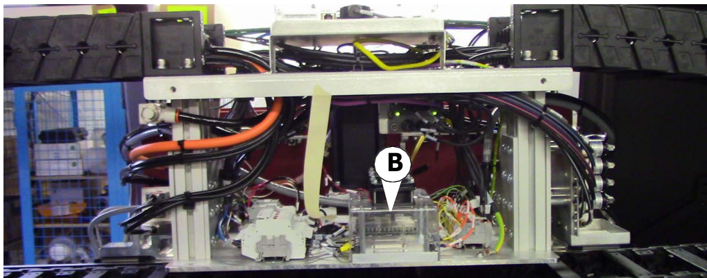
Figure 6-9 Power Supply Cooling Fan and Filter with Acrylic cover
