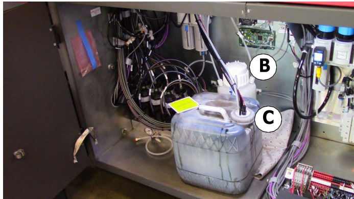
Figure 4-18 Waste container compartment
