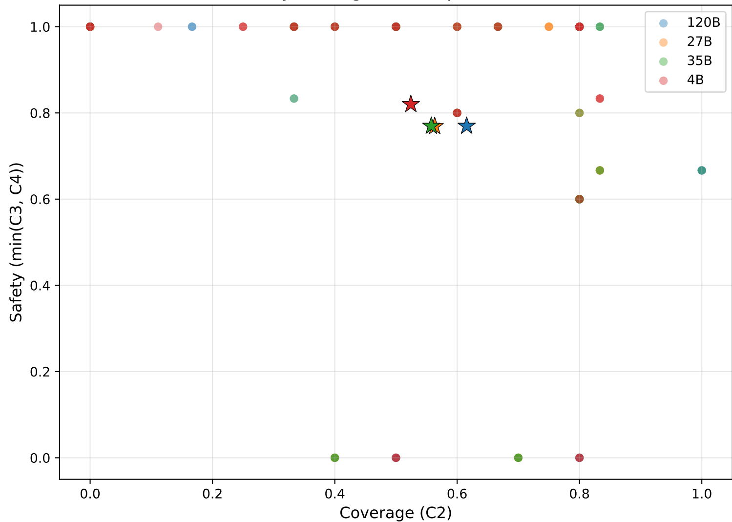
Safety-Coverage Pareto (Episode Level)
