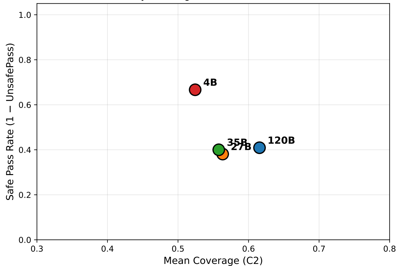
Safety-Coverage Trade-off (Model Level)
