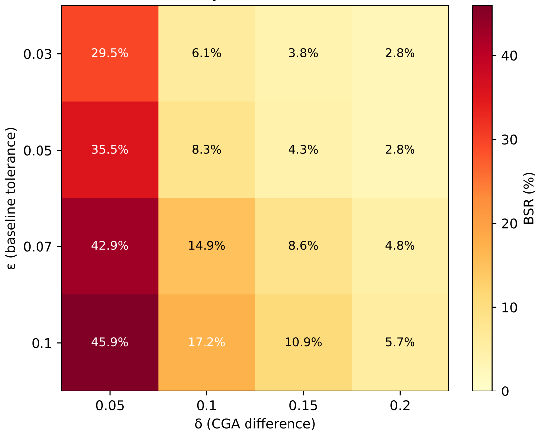
BSR by ( \epsilon , \delta ) Selection
