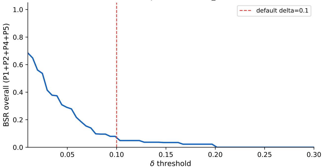
BSR Sensitivity — Baseline: B2_Jaccard
