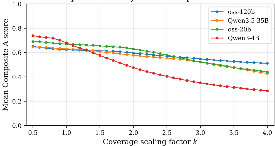
k-space Sensitivity: Model Composite Scores
