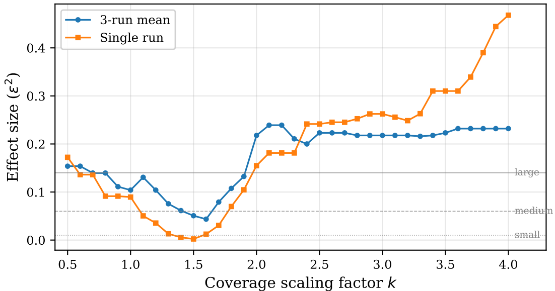
k-space Sensitivity: Effect Size Stability
