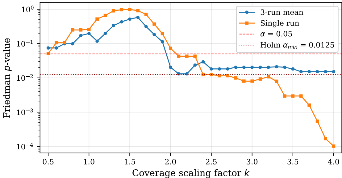
k-space Sensitivity: Friedman p -value Stability
