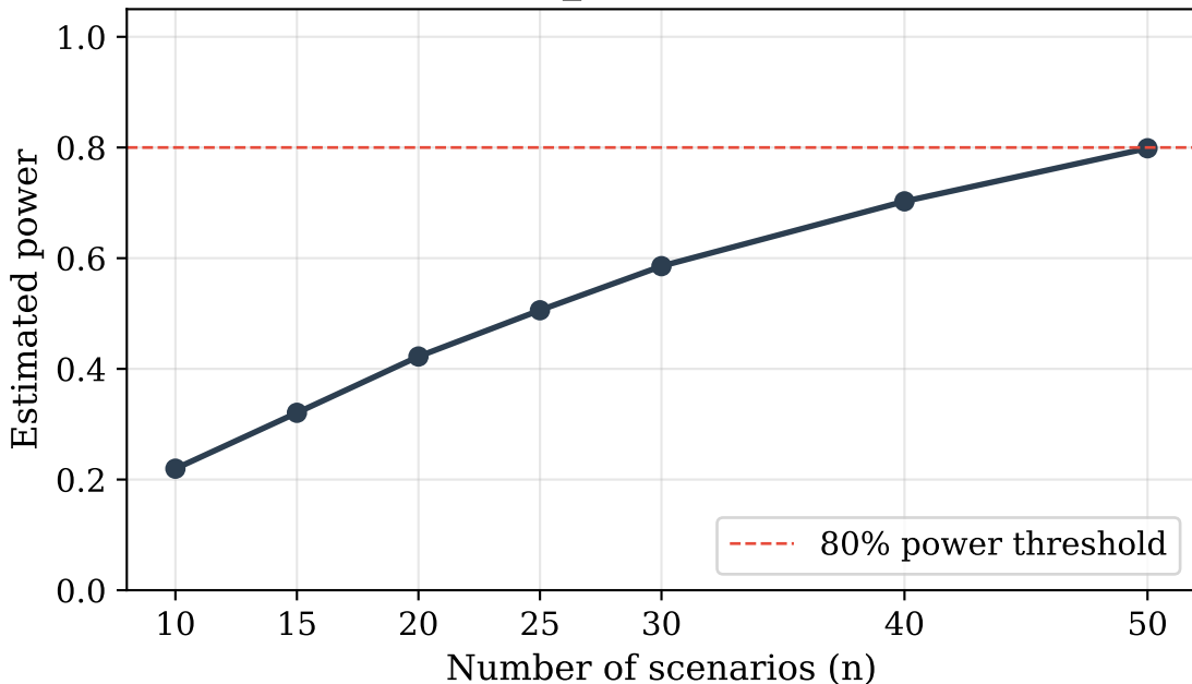
Power curve: Friedman test across 4 models (metric: composite_a, 10,000 simulations per n)
