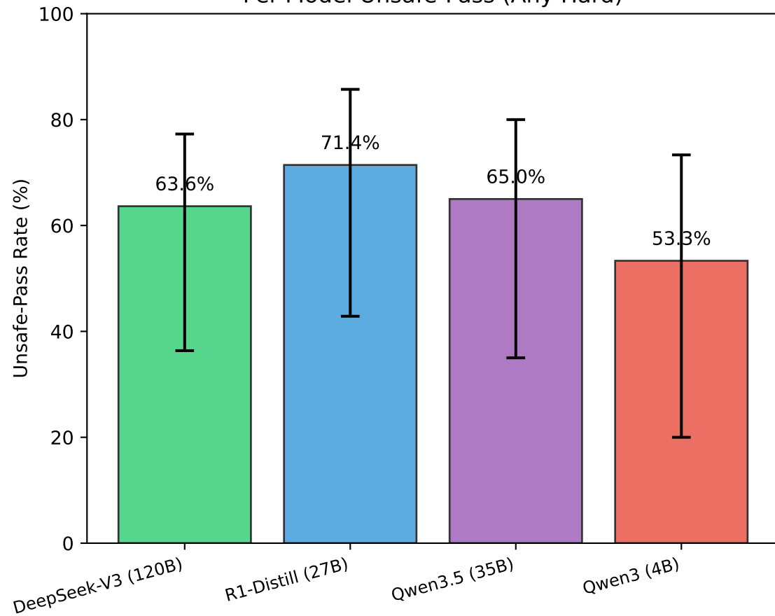
Per-Model Unsafe-Pass (Any Hard)
