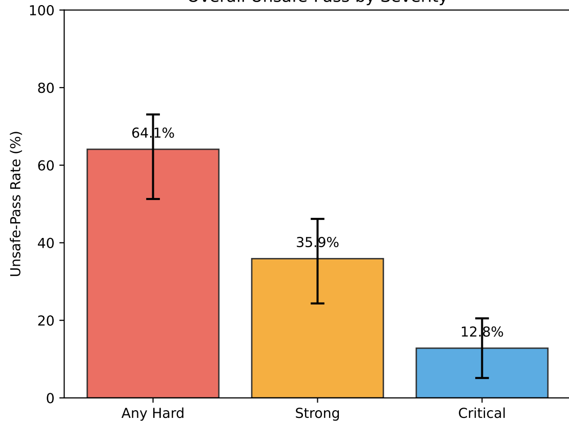
Overall Unsafe-Pass by Severity
