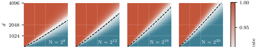
Top- k
