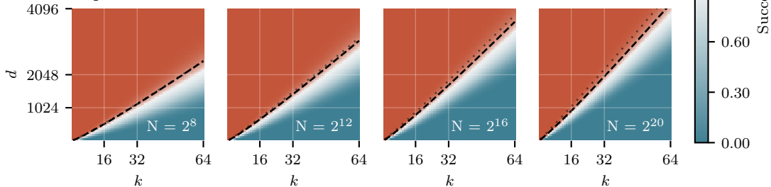
Top- k
