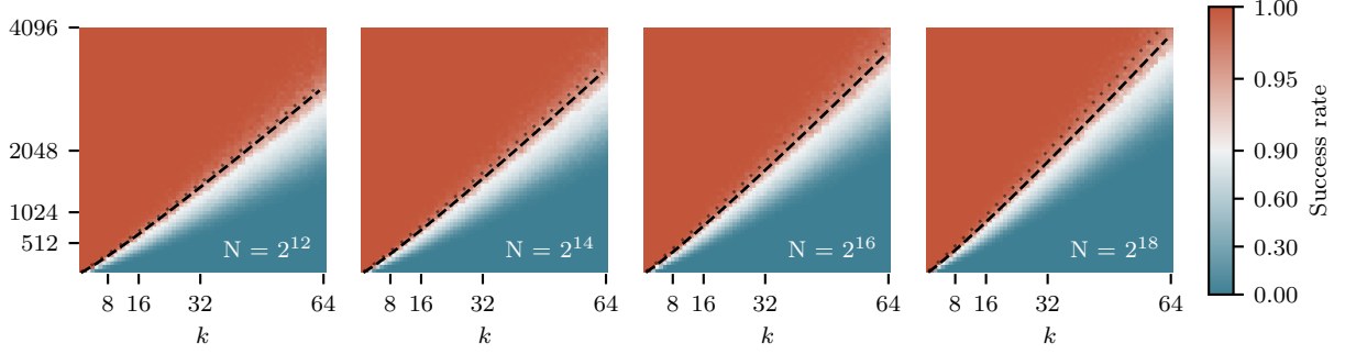
Figure 3: The prediction of Proposition 4 agrees well with numerical experiments.
