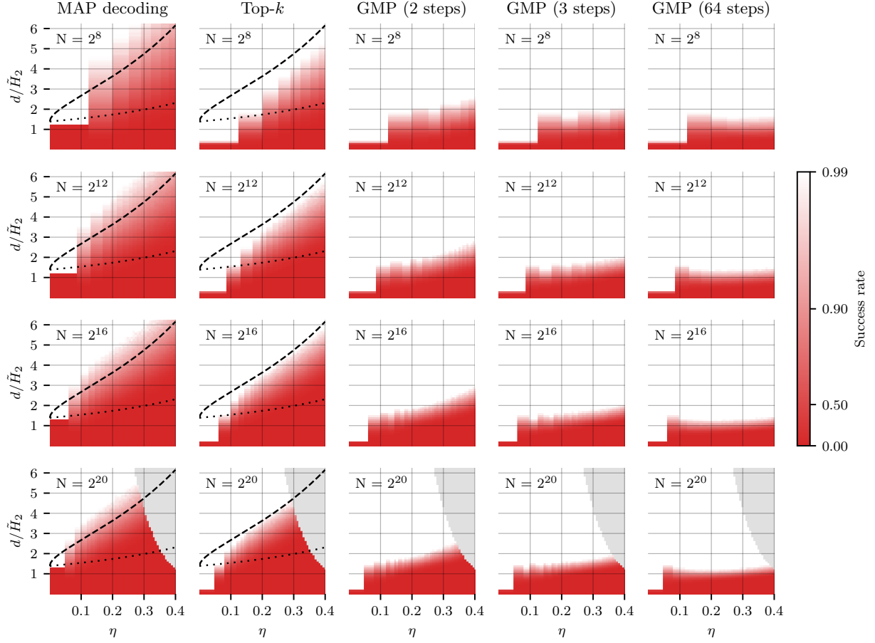
Figure 5: How many dimensions do we need to store one bit of information? We graph empirical performance of MAP thresholding, top- k , and gmp at exactly decoding a superposition code as a function of approximate inverse bitrate d/\tilde{H}_2 = d/(k \log_2(eN/k)) and sparsity exponent \eta = \ln k / \ln N . The dashed and dotted lines, respectively, plot the upper and lower bounds appearing in Corollary 2.
