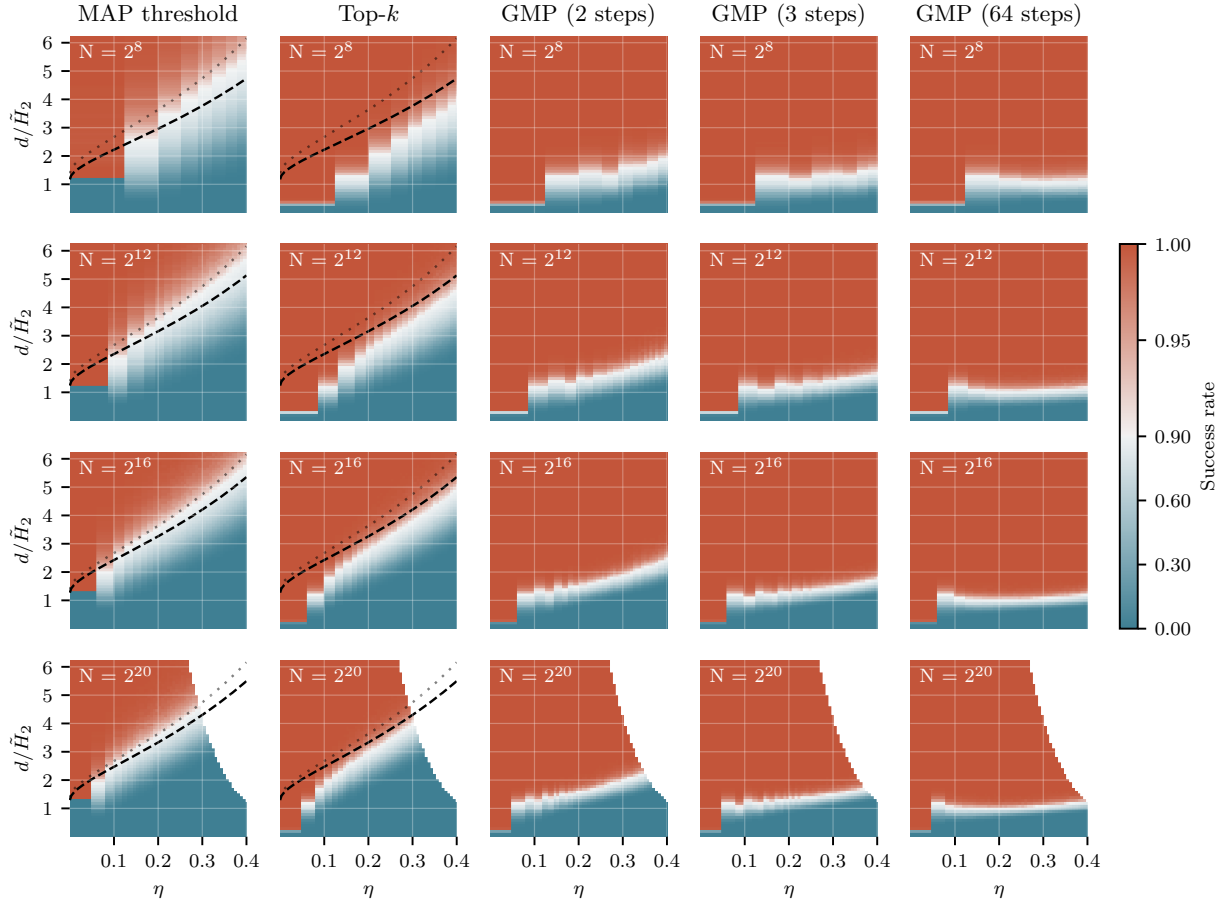
(b) How many dimensions do we need to store one bit of information? We graph empirical performance of MAP thresholding, top- k , and GMP at exactly decoding a superposition code as a function of approximate inverse bitrate d/\tilde{H}_2 = d/(k \log_2(eN/k)) and the sparsity exponent \eta = \ln k / \ln N . The bold line shows the critical value d = 2(1 + \sqrt{\eta})^2 k \ln N predicted by Proposition 4 and thin line shows the limit described in Corollary 1 as N \rightarrow \infty . In all cases, we use a dictionary of random spherical codewords.
