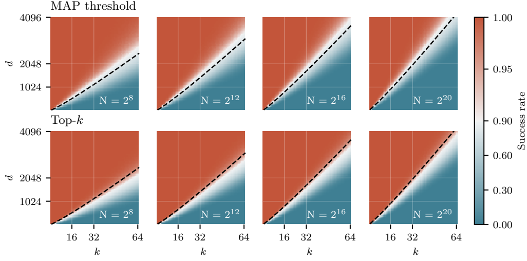
(a) Empirical performance of MAP thresholding and top- k thresholding at decoding a k -element subset of [N] from a d -dimensional superposition code using a random spherical dictionary. The dashed line shows the critical value d = 2(1 + \sqrt{\eta})^2 k \ln N predicted for threshold decoding by Proposition 4.
