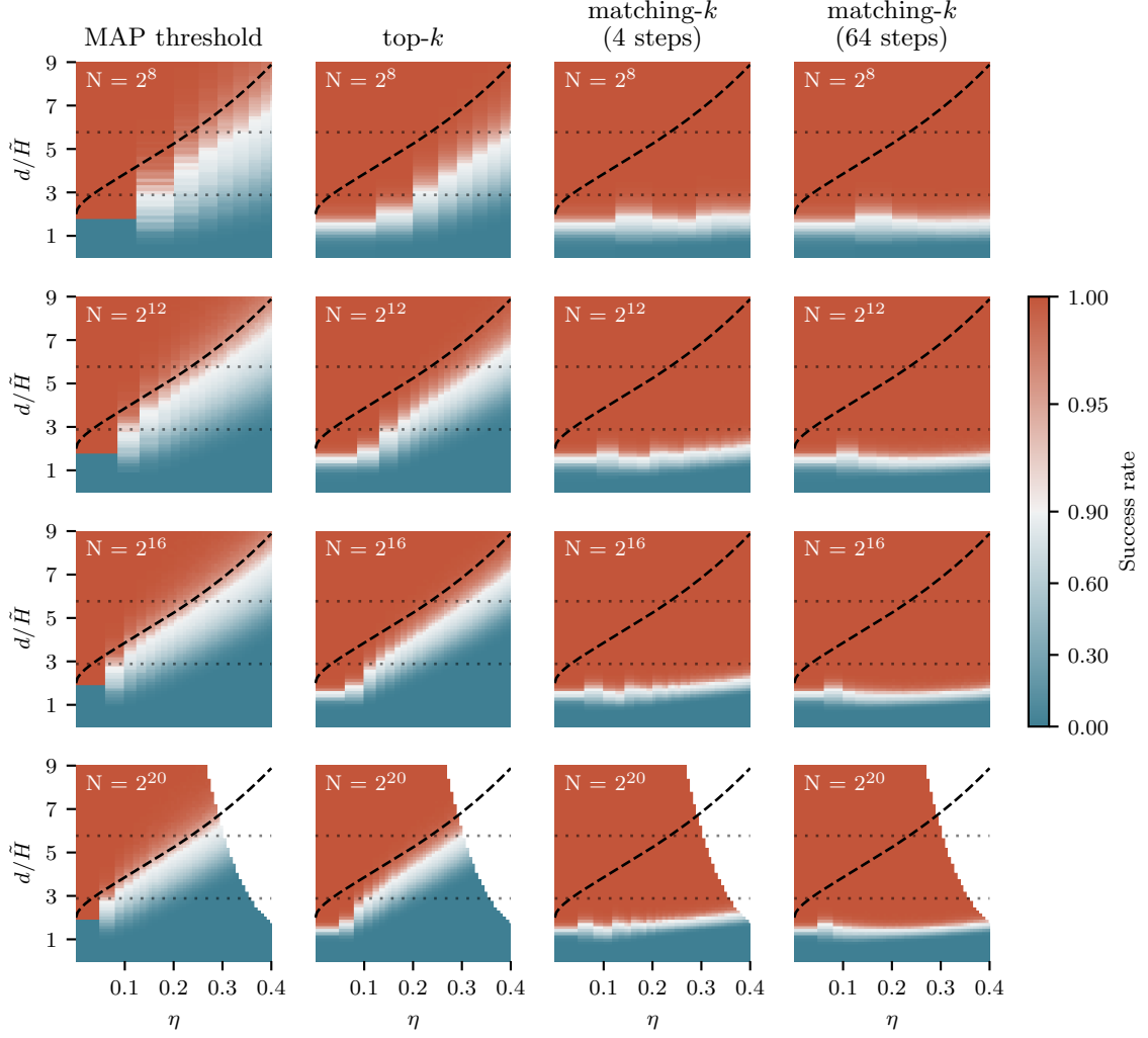
Figure 4: Empirical success rates of four different sparse recovery metrics at recovering a superposition code. Each graph shows
