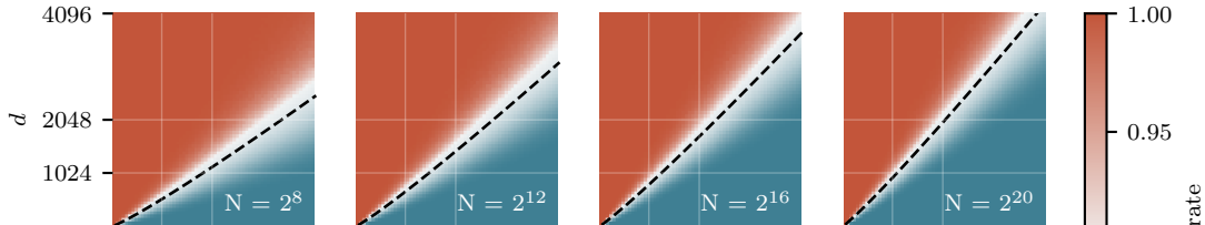
Top- k
