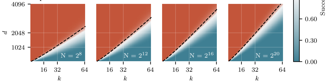
Top- k
