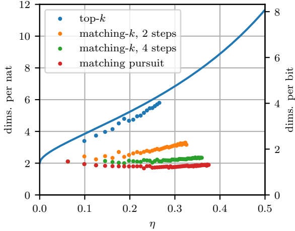
Figure 3: Solid line: effective inverse capacity guaranteed for top- k decoding by Proposition 4, graphed as a function of \eta = \ln k / \ln N . Points:
