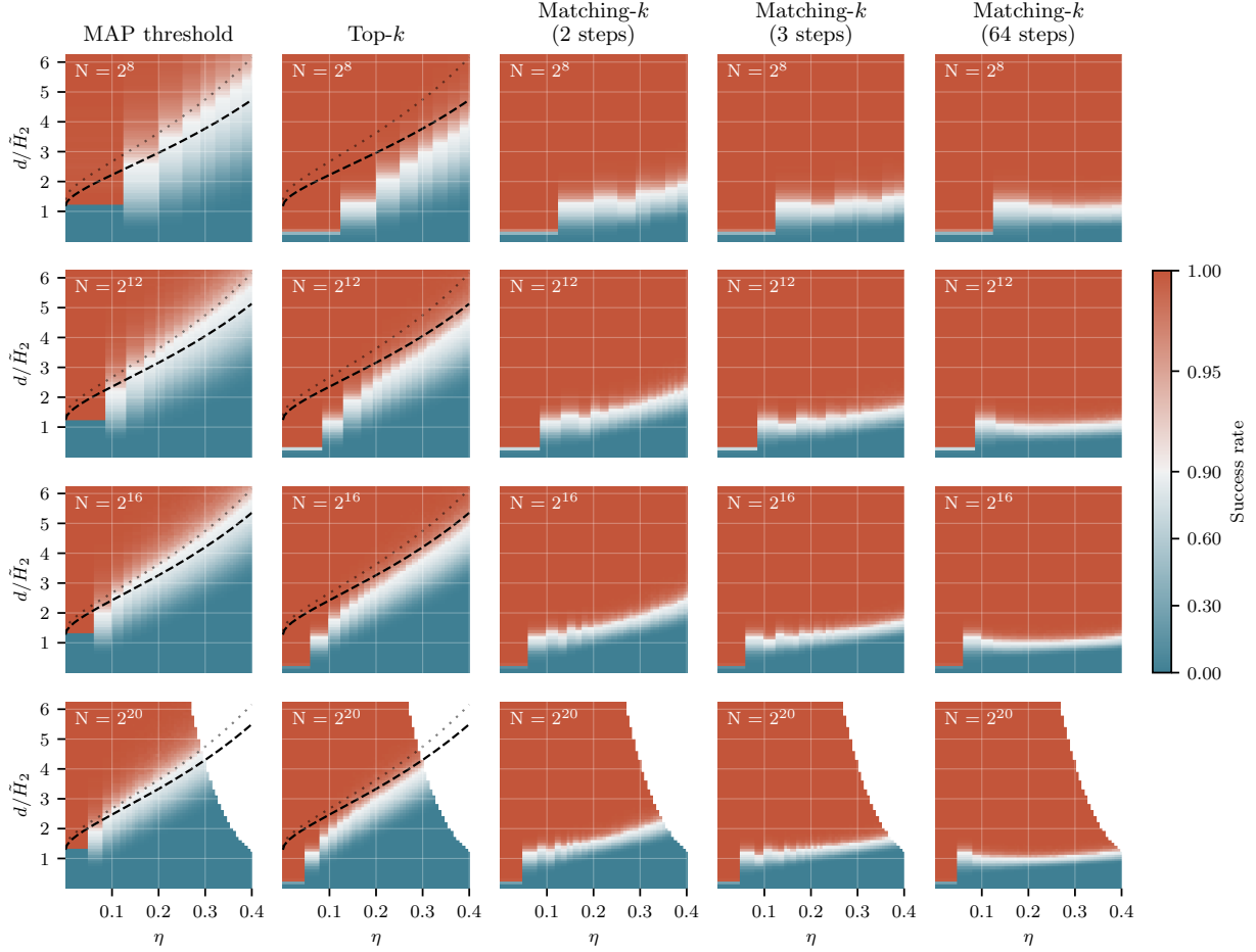
Figure 4: Empirical success rates of different sparse recovery methods at recovering a superposition code, graphed as a function of inverse bitrate d/\tilde{H}_2 = d/(k \log_2(eN/k)) and the sparsity exponent \eta = \ln k / \ln N . The bold line shows the “rule of thumb” for MAP thresholding derived from Proposition 4 and the thin line shows the limit of the bold line for large N .
