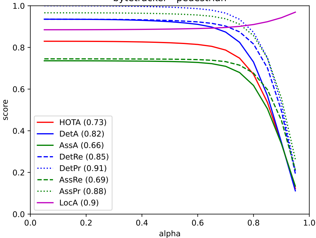
bytetracker - pedestrian
