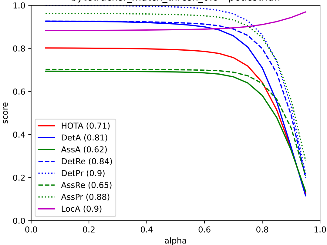
bytetracker_match_thresh_0.8 - pedestrian
