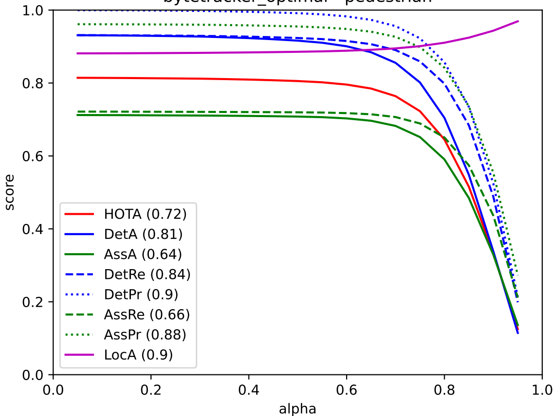
bytetracker_optimal - pedestrian
