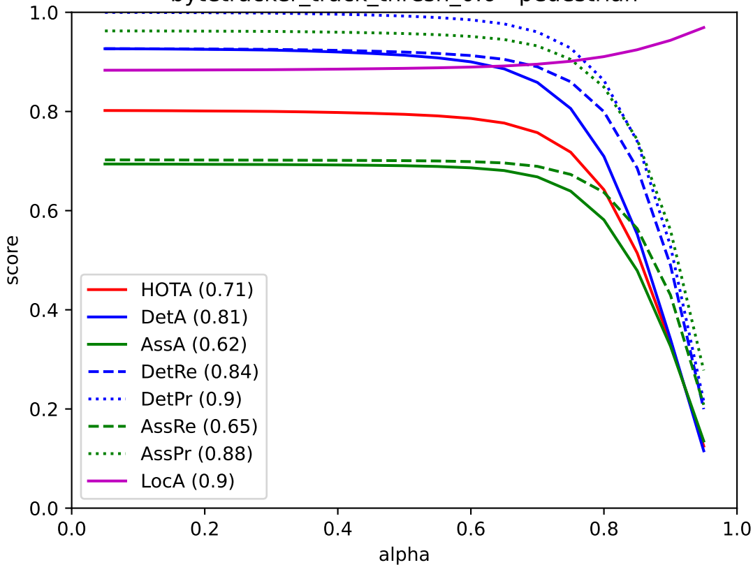
bytetracker track thresh 0.6 - pedestrian
