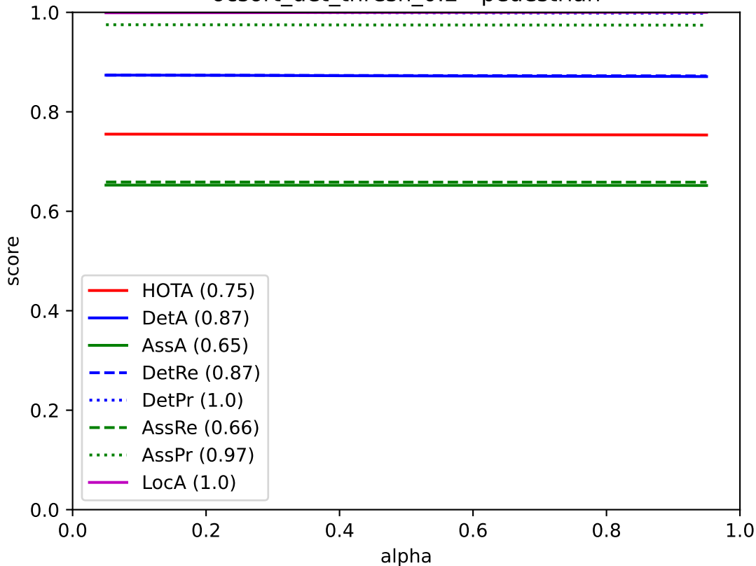
ocsort_det_thresh_0.2 - pedestrian
