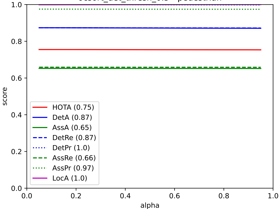
ocsort_det_thresh_0.5 - pedestrian
