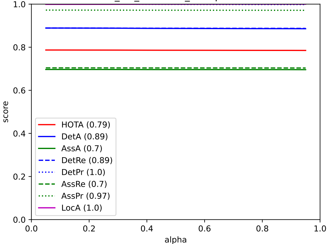
ocsort_iou_threshold_0.2 - pedestrian
