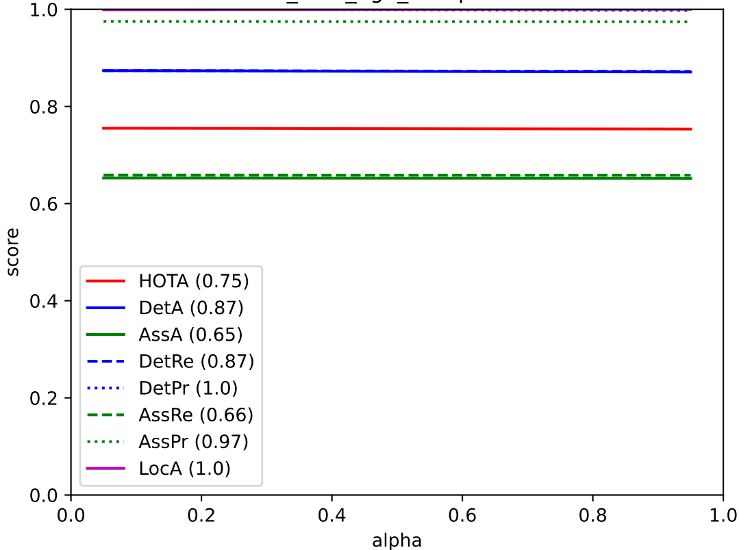
ocsort_max_age_30 - pedestrian
