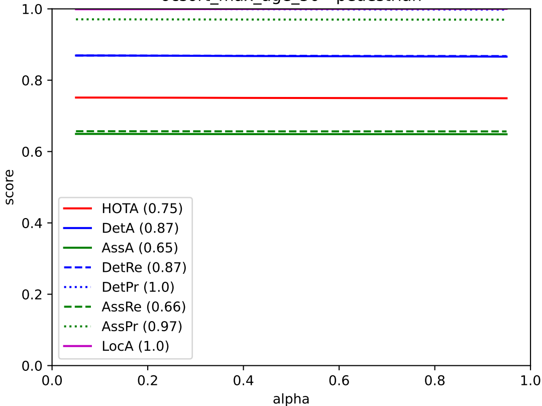
ocsort_max_age_50 - pedestrian
