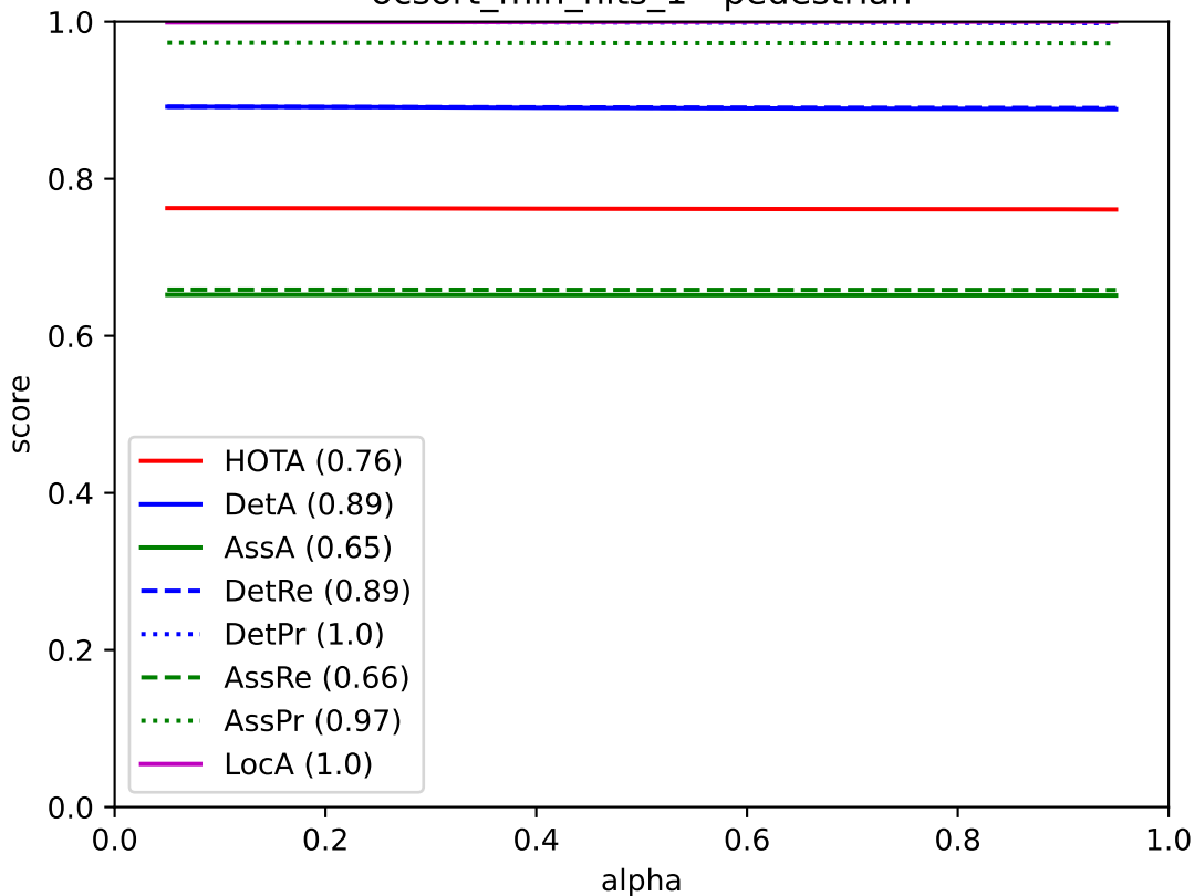
ocsort_min_hits_1 - pedestrian
