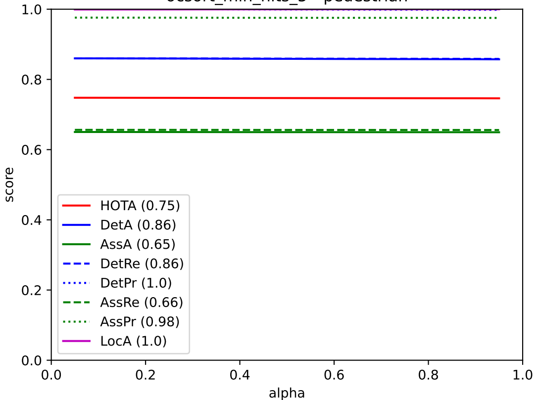
ocsort_min_hits_5 - pedestrian
