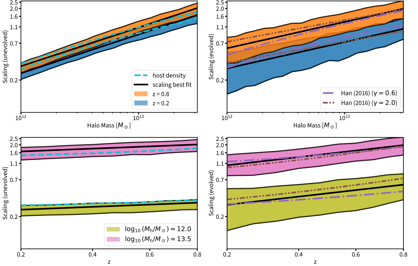
FIG. 4. The scaling shows the ratio of number of subhalos with mass 8 < \log_{10} m < 9 projected within an annulus with an inner and outer radius of 10 and 20 kpc respectively to the number of these subhalos in a 10^{13} M_{\odot} host halo at z = 0.5 as a function of host halo mass and redshift. The scaling value and its scatter are calculated by using the mean and standard deviation over all host halos. The left panels show the unevolved subhalo scaling, while the right panel shows the scaling of the evolved distribution. Upper panels show the halo mass scaling relation for host halos at redshift z = 0.2 (blue) and z = 0.8 (orange). Lower panels show the redshift scaling relation for a host halo mass of 10^{12.0} M_{\odot} (olive) and 10^{13.5} M_{\odot} (pink). Shaded regions show the 1\sigma halo to halo scatter. The unevolved scaling is compared to the scaling of the host's density profile (adjusted to the definition of halo mass used here) in blue (dashed). The scaling relations derived from the Han et al. [21] analytic number density distribution (Eq. 1 and 5) are shown for \gamma = 0.6 (purple, dot dashed) and \gamma = 2.0 (brown, dot dashed). These values of \gamma span a range of physically plausible values.
