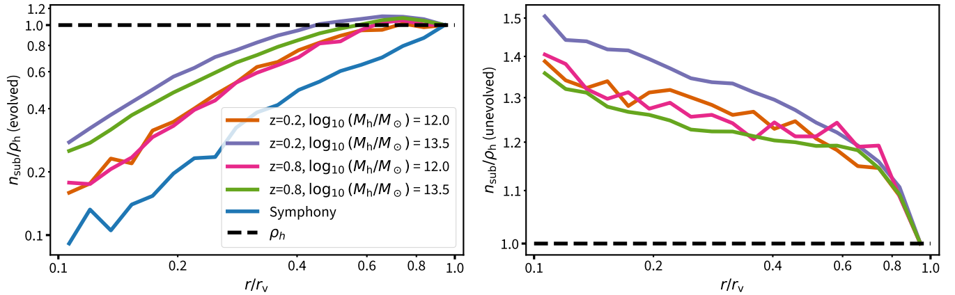
FIG. 2. The ratio of the spatial distribution of subhalos ( n_{\text{sub}} ) to the host's density profile ( \rho_h ) for subhalos with 8 < \log_{10}(m_b/M_\odot) < 9 normalized to 1 at r = r_v for the evolved distribution (left) and 8 < \log_{10}(m_b/M_\odot) < 9 unevolved distribution (right). A horizontal line of 1 (black dotted) shows the host halos density profile. Results are plotted for galacticus over a range of host halo masses and redshifts and for Symphony for a single mass and redshift ( \log_{10}(M_h/M_\odot) = 13, z = 0.5 ). The relative decrease towards the center in the evolved case is a result of tidal stripping (see Section II B), while the relative increase in the unevolved case is likely a result of dynamical friction (see Section IV A). Over our range of redshifts explored by our galacticus simulations, the slope of the evolved spatial distribution n_{\text{sub}}/\rho_h has a mild dependence on halo mass, with almost no dependence on redshift. For the unevolved case, there appears to be no significant dependence on either redshift or host halo mass.
