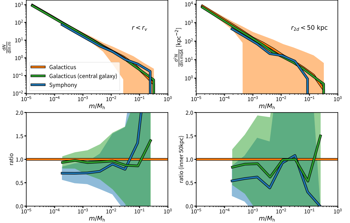
FIG. 5. Upper left: the SHMF over the entire virial volume, right: the SHMF for subhalos projected within 50 kpc. Results are shown for group mass halos ( M_h \sim 10^{13} M_\odot ) at redshift z = 0.5 . The galacticus DMO predictions are shown in orange, galacticus predictions for the central galaxy are shown in green, and results for the Symphony suite are shown in blue. Lower left and right show the ratios to the galacticus DMO predictions. The effect of the central galaxy can be seen as a reduction in normalization of the SHMF no significant change to the logarithmic slope, at least for low mass halos. The galacticus and Symphony mass function and its halo to halo scatter are calculated by taking the mean and standard deviation of the value of the mass functions of every halo at every mass bin (in the upper panel, only the the galacticus DMO scatter is shown for clarity). For the lower panels, the values of the ratio and its scatter are calculated by dividing the average mass function and its scatter by the average value of the galacticus DMO mass function at each mass bin. Note that the difference in normalization for galacticus with and without a central galaxy is significantly less than the difference between our galacticus models and the Symphony dark matter only simulation suite.
