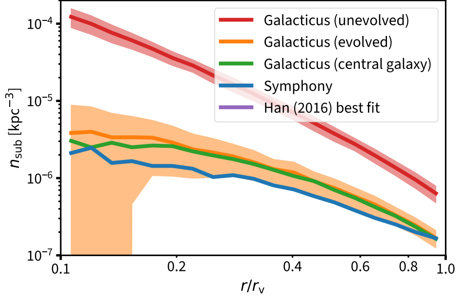
FIG. 1. The differential spatial distributions ( n_{\text{sub}} ) from our galacticus models and Symphony for subhalos with mass 9 < \log_{10}(m_b/M_\odot) < 10 plotted as a function of the virial radius fraction ( r/r_v ). Results are for halos with mass M_h = 10^{13} M_\odot at redshift z = 0.5 . In red: the unevolved spatial distribution from our galacticus models, in orange: the evolved spatial distribution for galacticus and in green with a central galaxy. The galacticus and Symphony spatial distributions shown are a result of averaging over the spatial distributions of each individual halo in the suite at each bin over all halos in the suite. The halo to halo scatter is calculated in a similar way; taking the standard deviation of the values of the spatial distributions of each of the host halos calculated at each radial bin. The shaded regions show the 1\sigma halo to halo scatter for the galacticus evolved and unevolved case, scatter for the other distributions is not shown for visual clarity. The best fit of the Han (2016) model to the galacticus DMO unevolved spatial distribution is shown in purple. In blue: the spatial distribution for Symphony. We find there is no significant difference in the spatial distribution of subhalos when running models with or without a central galaxy.
