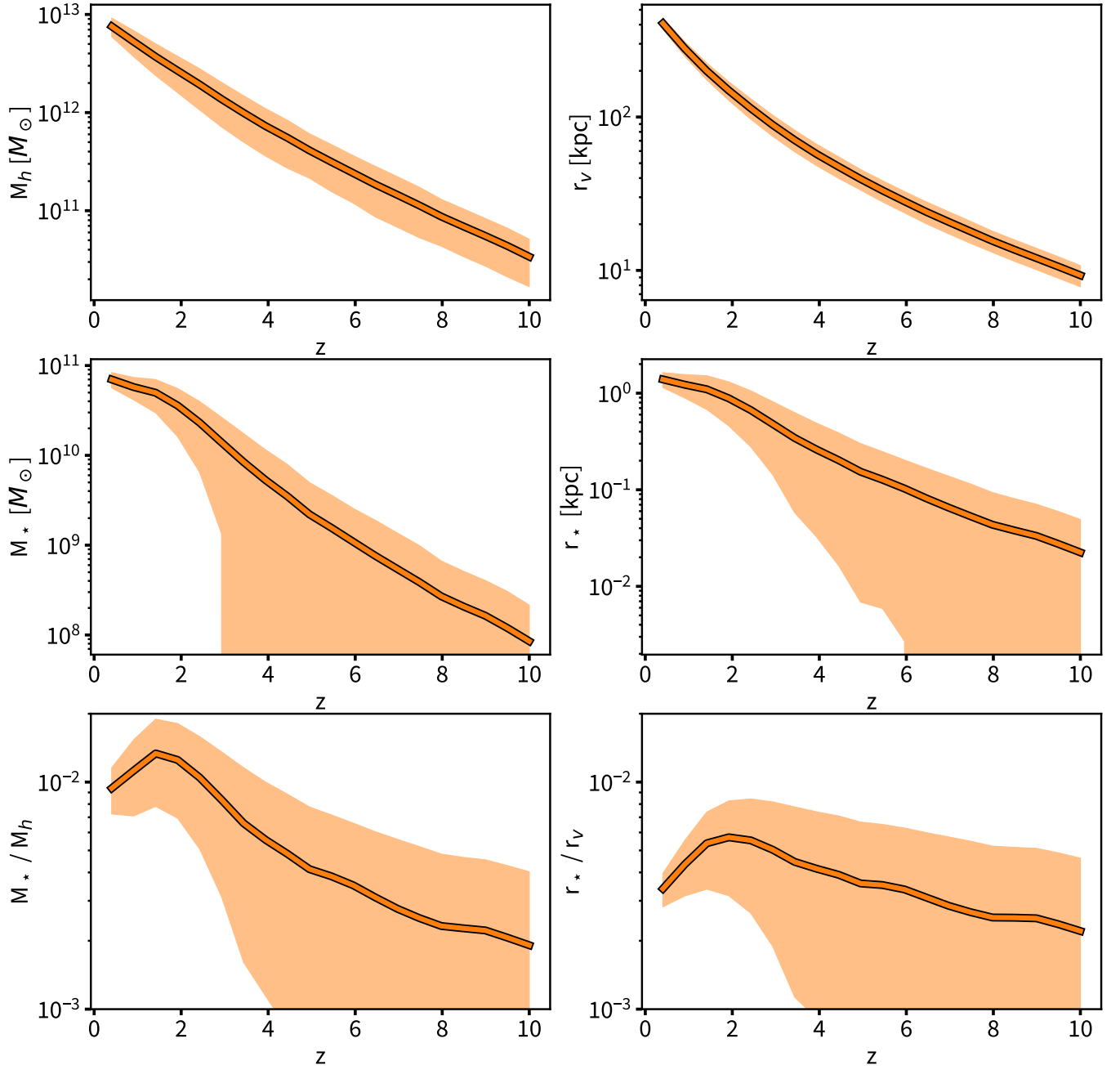
FIG. 6. Our galacticus model predictions for the evolution of a 10^{13} M_{\odot} halo and its central galaxy. Stellar masses are determined using the Behroozi et al. [35]. relation between halo mass and stellar mass, while galactic radii are determined using empirical fits to the stellar mass to stellar radius relation provided by Shen et al. [54]. For simplicity, no scatter has been included in either of these relationships. The top left panel gives the evolution of the mass of the central halo while the top right panel gives the evolution of the virial radius of the halo. The middle left panel shows the evolution of the stellar mass, while the middle right panel shows the evolution of the Hernquist radius of the central galaxy. Finally, the lower left and right panels show the evolution of the ratio of stellar mass to halo mass and Hernquist radius to virial radius, respectively. The curve shows the mean value, while the shaded region shows 1\sigma scatter.
