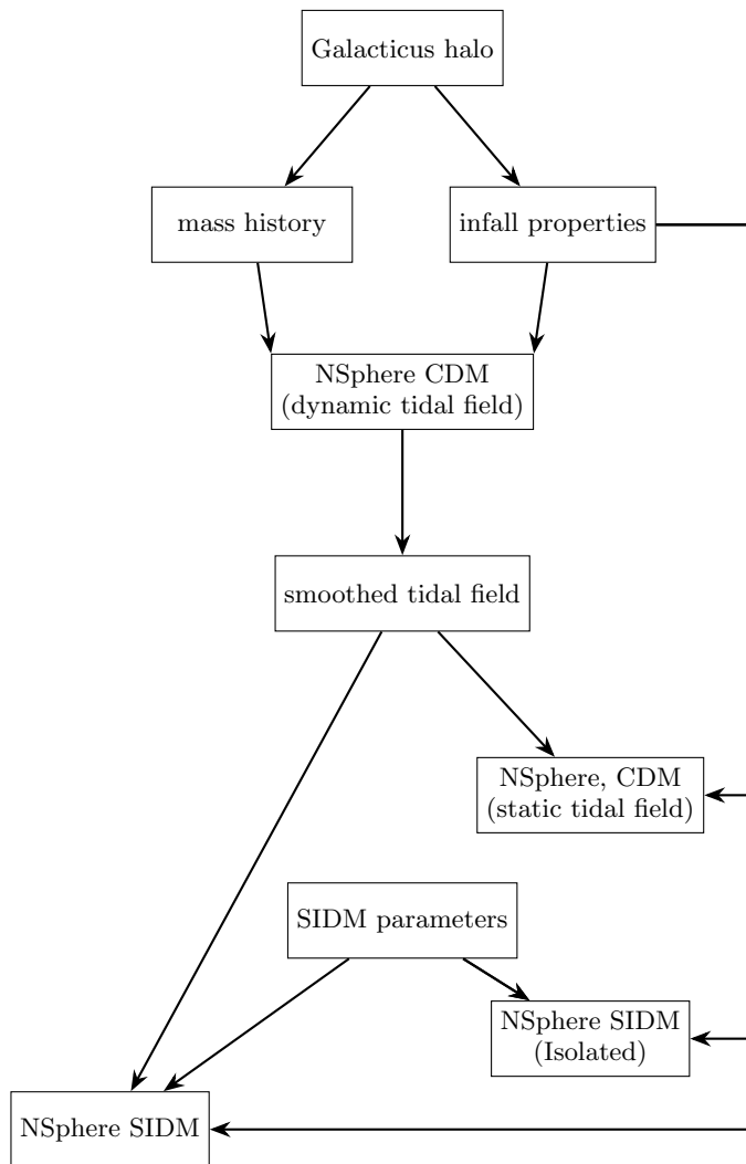
FIG. 1. A diagram of the T1DES pipeline simulating a single subhalo. The T1DES pipeline begins with extracting infall properties ( r_s , r_v , z_{infall} ) as well as the bound mass of the subhalo as a function of time. Our main results use the galacticus galaxy formation model to extract the infall mass properties of the subhalo, however we also include results using properties extracted from N-body simulations. These are used to set the initial conditions of the halo and begin running a first pass of NSphere in “dynamic” tidal field mode. During this run, NSphere calculates a tidal field “in flight” that results in a mass history approximating that of the galacticus halo. After the run, the tidal field is then smoothed on the scale of the dynamical time of the subhalo to remove the rapid variations in the initial calculation of the tidal field. For comparison, we rerun NSphere in CDM mode to get a “replay” of the subhalo’s evolution using the smoothed tidal field. Then we run NSphere in SIDM mode with the smoothed tidal field. Finally, for comparison we run a NSphere SIDM on an isolated halo corresponding to the infall properties of the subhalo.
