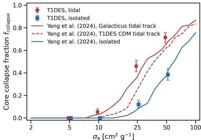
FIG. 4. The cross section per unit mass vs the core collapse fraction for our T1DES simulations compared to as well as predictions from [17]. In red: results from our tides subhalo simulations (red dot with error bars), and the Yang models integrated over the the tidal tracks from galacticus (red solid) and from the T1DES CDM (red dotted) in blue. We find our T1DES model is fairly consistent with the predictions from the [17] model, though our T1DES model may predict slightly higher fractions of core collapsed halos. In blue is the results for the isolated case, if the subhalos remained isolated, what fraction would collapse? Our T1DES model is consistent with the predictions of the Yang model here and predicts strictly lower collapse fractions for isolated halos. No halos collapse in the field that also do not collapse as a subhalo.
