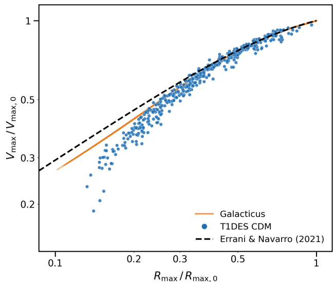
FIG. 3. We plot the normalized tidal tracks from our T1DES CDM smoothed stage simulations, our galacticus models and from the empirical Errani and Navarro [44]. For each subhalo in our suite, we plot the R_{\text{max}}/R_{\text{max},0} and V_{\text{max}}/V_{\text{max},0} at the subhalo's apocenter where R_{\text{max},0} and V_{\text{max},0} are the initial R_{\text{max}} and V_{\text{max}} of the subhalo at apocenter. We plot the Normalized tidal tracks from galacticus , T1DES and predictions. When properly normalized, CDM tidal tracks are expected to follow a near universal relation. We find general good agreement on the tidal track level between our simulations; with slight disagreement for low R_{\text{max}} and V_{\text{max}} .
