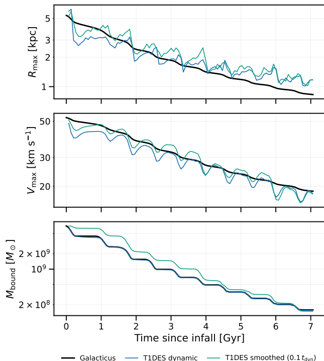
FIG. 2. The evolutionary history of an example CDM T1DES subhalo and its galacticus counterpart. We show the bound mass history, M_{\text{bound}} as well as the internal properties of the subhalo, R_{\text{max}} and V_{\text{max}} (see Eq. 7). Each sudden drop in the mass history corresponds to a peri-centric passage of the subhalo, this subhalo completes 10 pericentric passages in its 7Gyr evolution within the host, losing \sim 90\% of its mass since infall. Results from both T1DES stages are shown: results from the T1DES dynamic stage, where the is dynamically calculated as well as the results from the T1DES dynamic stage, where we rerun with the dynamically calculated tidal field smoothed by a gaussian kernel. We note that while our model calculates a tidal field to match the provided galacticus mass history, it is not tuned to match the internal R_{\text{max}} and V_{\text{max}} properties; even so it is in good agreement with galacticus for nearly all halos.
