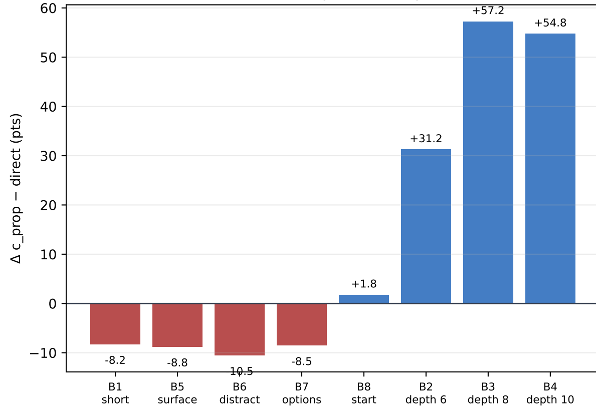
A1-bis vs adapted direct path
