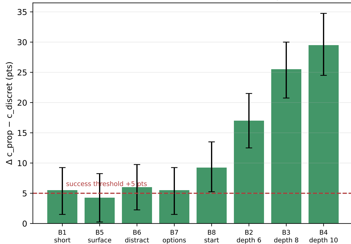
A1-bis vs discretisation (zero training)
