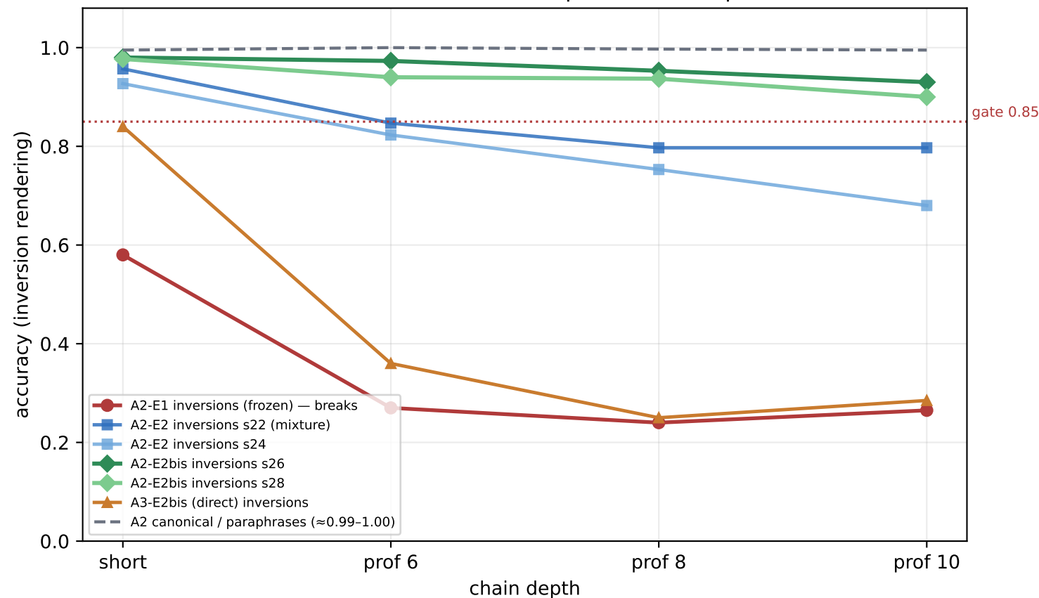
V2.3 → E2-bis: the crossed inversion×depth frontier is pushable with data
