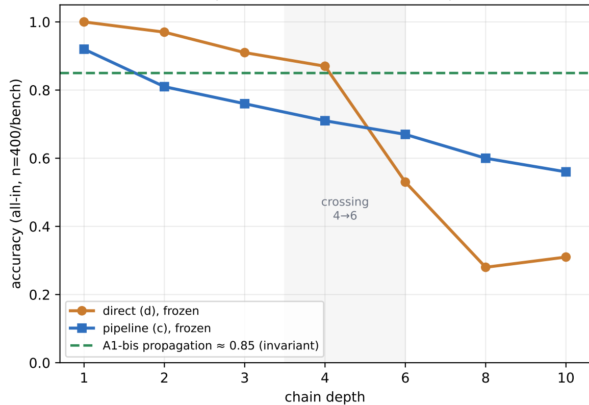
V2.1 depth reversal on frozen checkpoints
