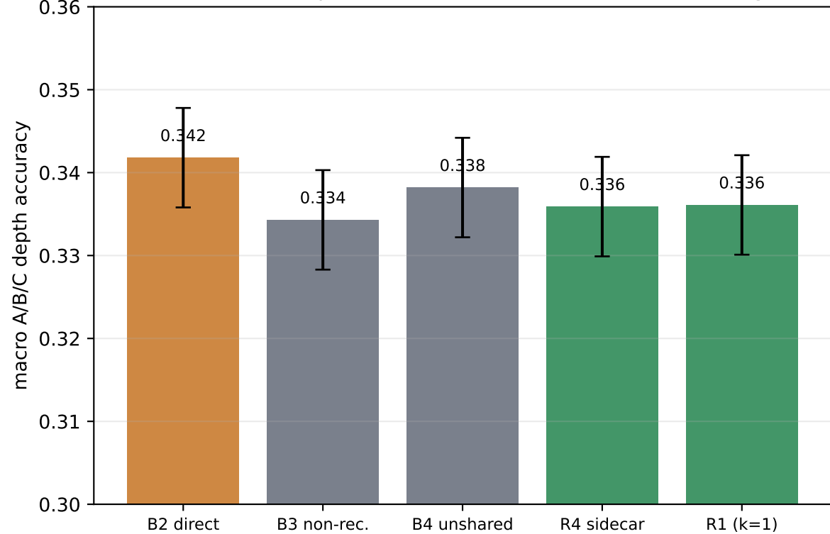
V1 reserved depth test (3 seeds): no sidecar advantage
