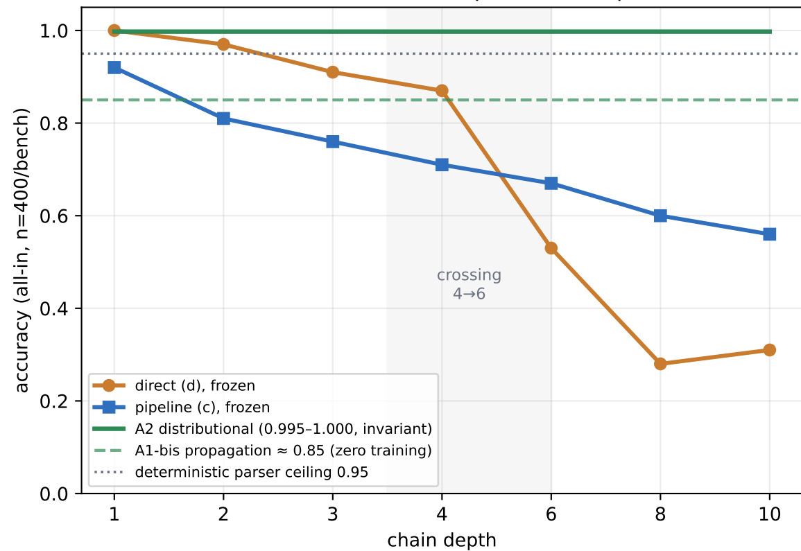
V2.1/V2.2 on frozen + repaired checkpoints
