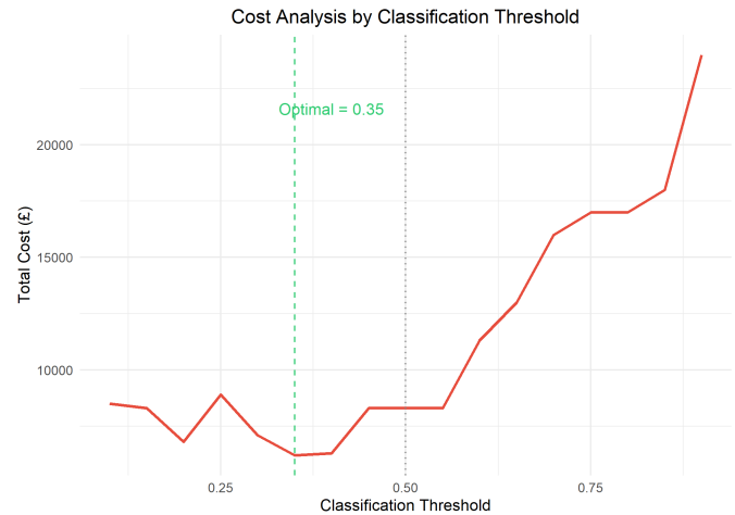
Fig. 2. Total misclassification cost by classification threshold (FN = £1,000, FP = £300). Optimal = 0.35, reducing cost by 25%.
